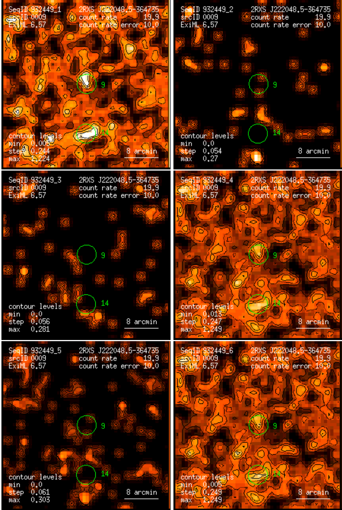
Figure 9: RASS 932449: detection 0009: band rate images, Gaussian filter: (1) PSPC channels 11 – 41, (2) 52 – 90, (3) 91 – 201, (4) 11 – 235, (5) 52 – 201, (6) 11 – 201. Broad band rates in counts/ks. Band rate contour levels in counts/ks/arcmin 2 .
