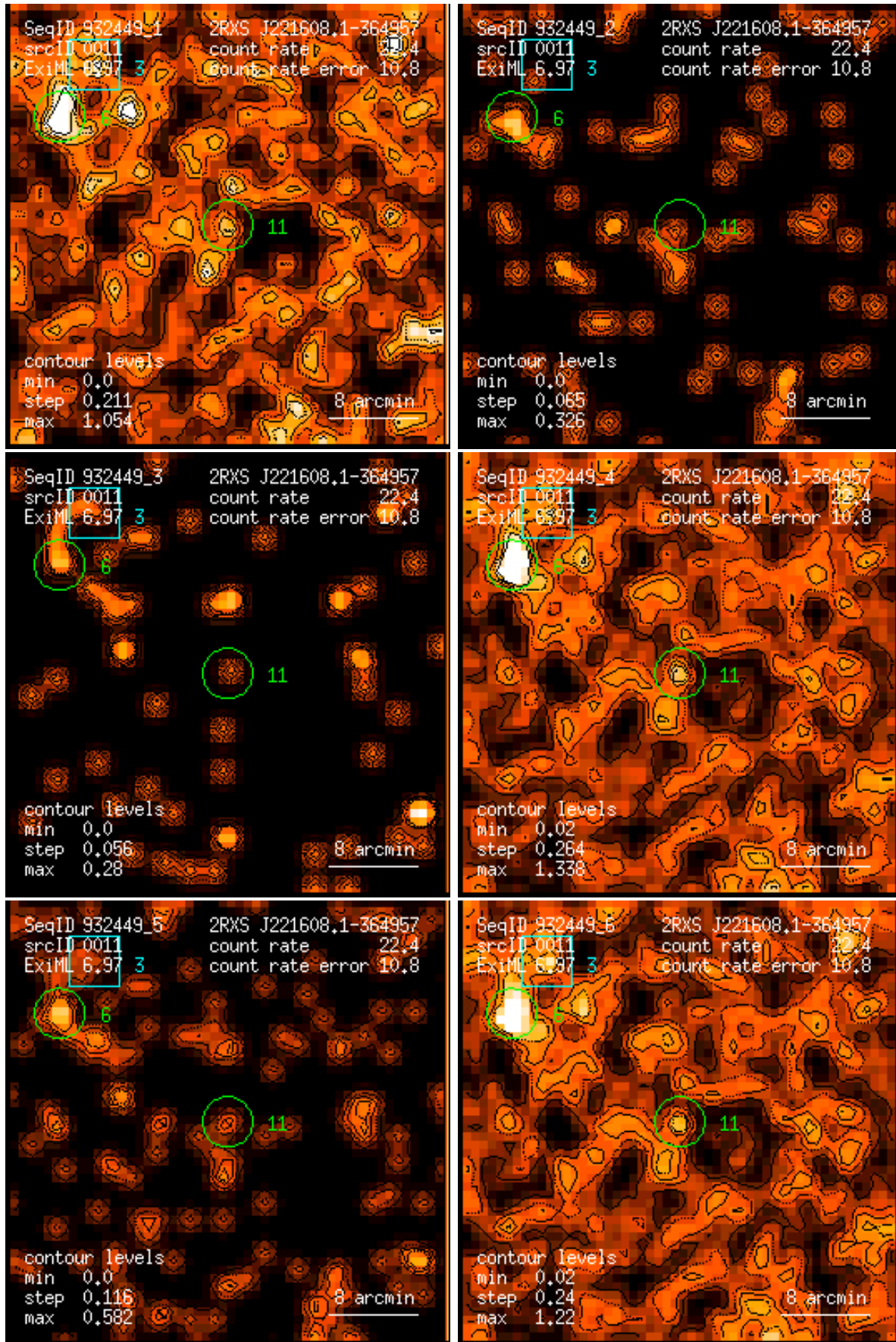
Figure 11: RASS 932449: detection 0011: band rate images, Gaussian filter: (1) PSPC channels 11 – 41, (2) 52 – 90, (3) 91 – 201, (4) 11 – 235, (5) 52 – 201, (6) 11 – 201. Broad band rates in counts/ks. Band rate contour levels in counts/ks/arcmin 2 .
