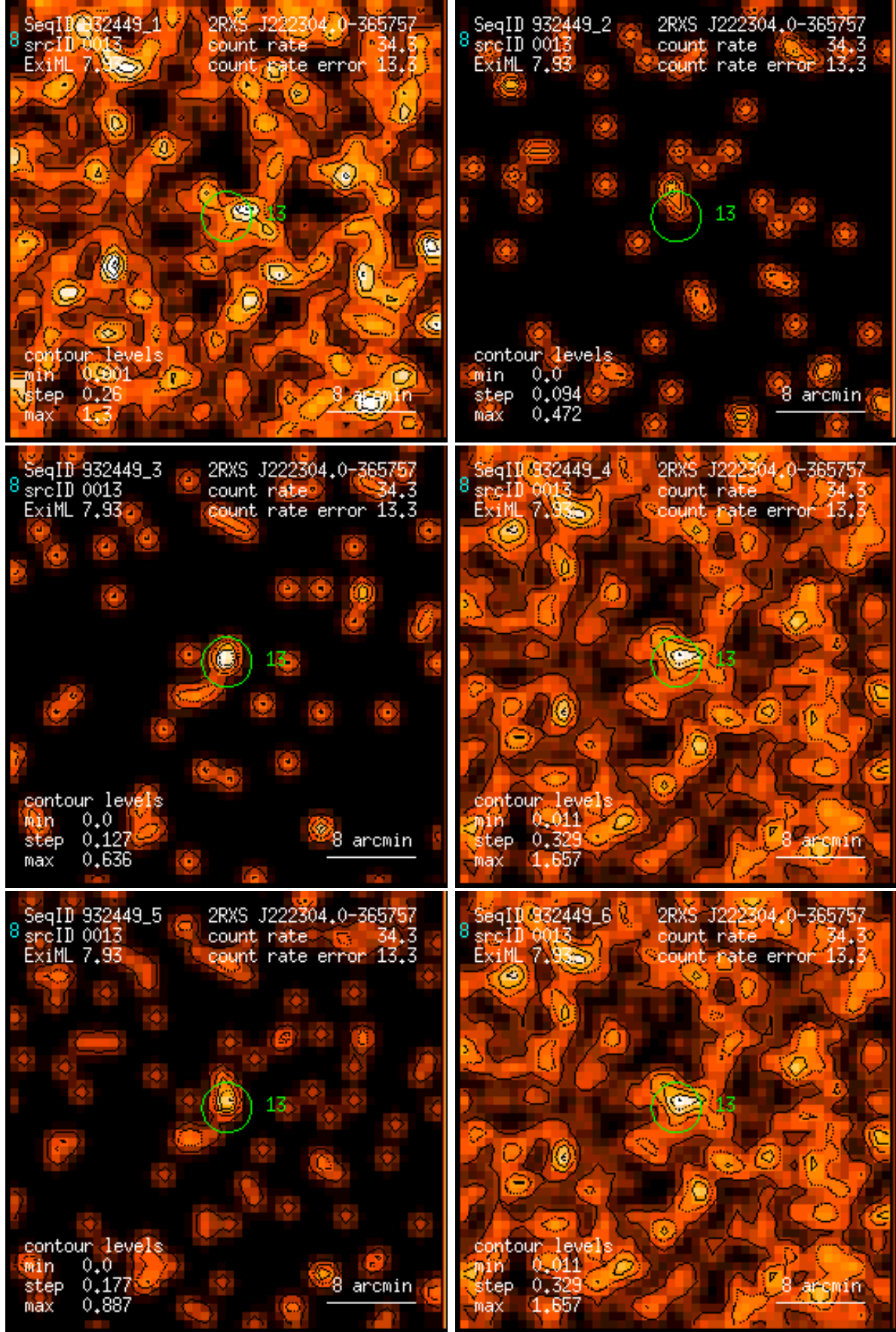
Figure 13: RASS 932449: detection 0013: band rate images, Gaussian filter: (1) PSPC channels 11 – 41, (2) 52 – 90, (3) 91 – 201, (4) 11 – 235, (5) 52 – 201, (6) 11 – 201. Broad band rates in counts/ks. Band rate contour levels in counts/ks/arcmin 2 .
