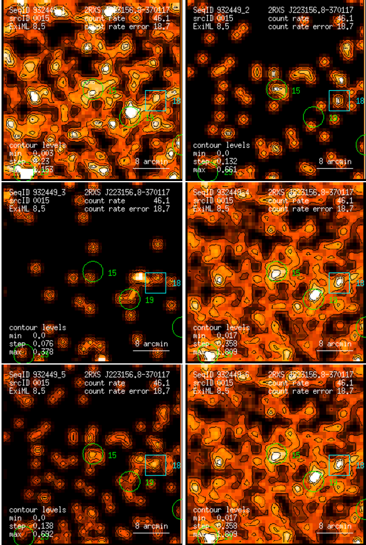
Figure 15: RASS 932449: detection 0015: band rate images, Gaussian filter: (1) PSPC channels 11 – 41, (2) 52 – 90, (3) 91 – 201, (4) 11 – 235, (5) 52 – 201, (6) 11 – 201. Broad band rates in counts/ks. Band rate contour levels in counts/ks/arcmin 2 .
