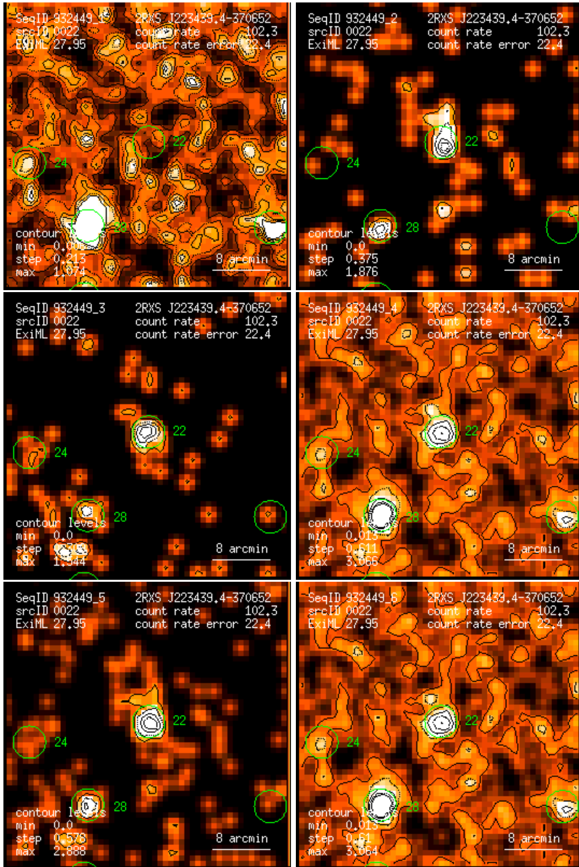
Figure 22: RASS 932449: detection 0022: band rate images, Gaussian filter: (1) PSPC channels 11 – 41, (2) 52 – 90, (3) 91 – 201, (4) 11 – 235, (5) 52 – 201, (6) 11 – 201. Broad band rates in counts/ks. Band rate contour levels in counts/ks/arcmin 2 .
