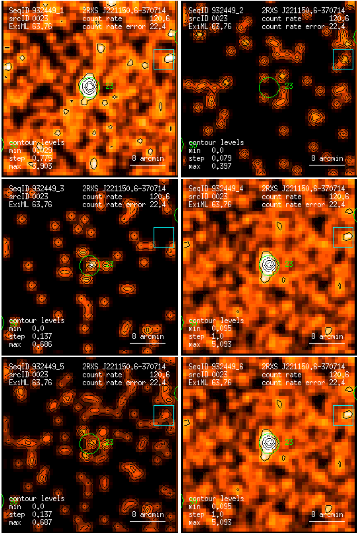
Figure 23: RASS 932449: detection 0023: band rate images, Gaussian filter: (1) PSPC channels 11 – 41, (2) 52 – 90, (3) 91 – 201, (4) 11 – 235, (5) 52 – 201, (6) 11 – 201. Broad band rates in counts/ks. Band rate contour levels in counts/ks/arcmin 2 .
