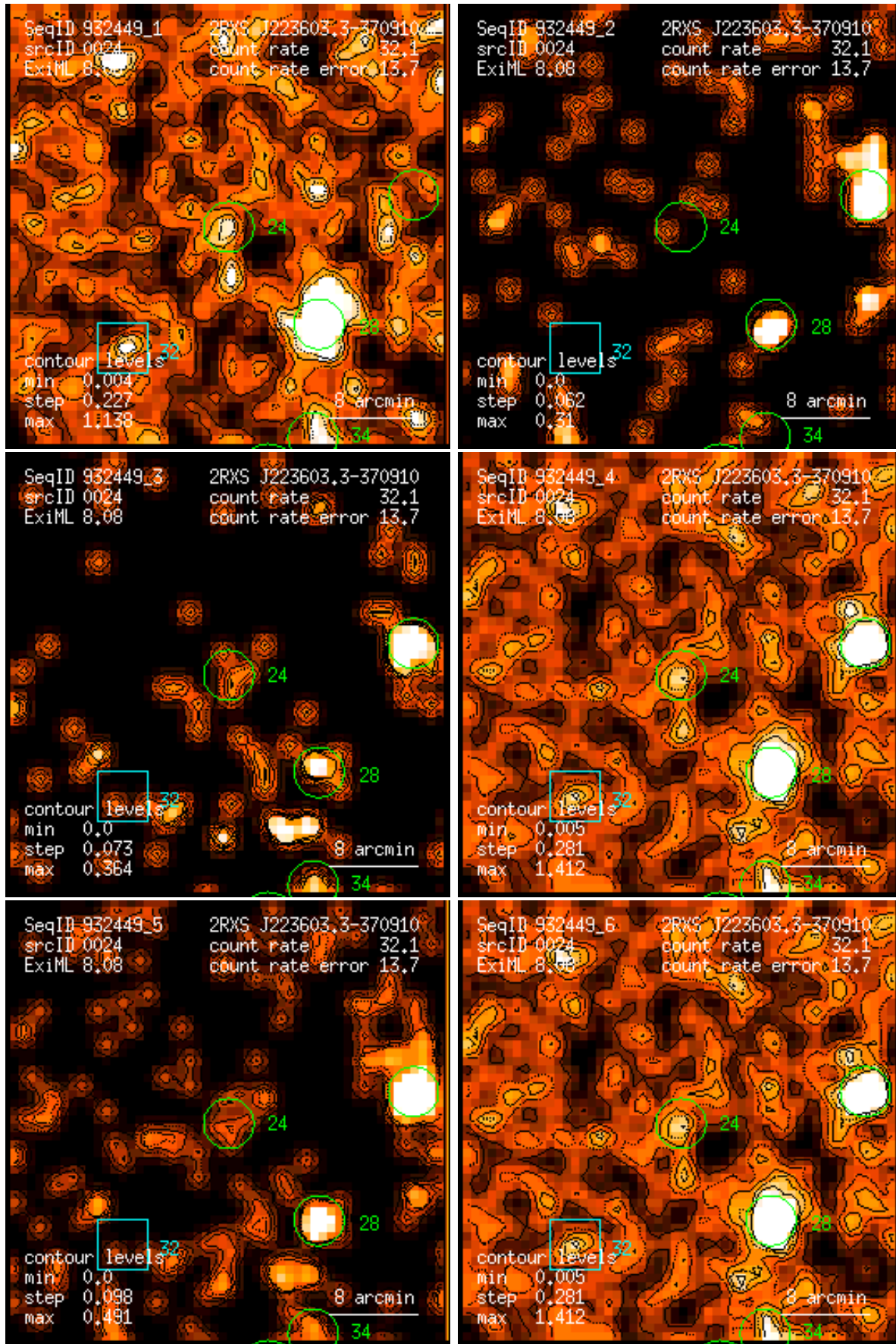
Figure 24: RASS 932449: detection 0024: band rate images, Gaussian filter: (1) PSPC channels 11 – 41, (2) 52 – 90, (3) 91 – 201, (4) 11 – 235, (5) 52 – 201, (6) 11 – 201. Broad band rates in counts/ks. Band rate contour levels in counts/ks/arcmin 2 .
