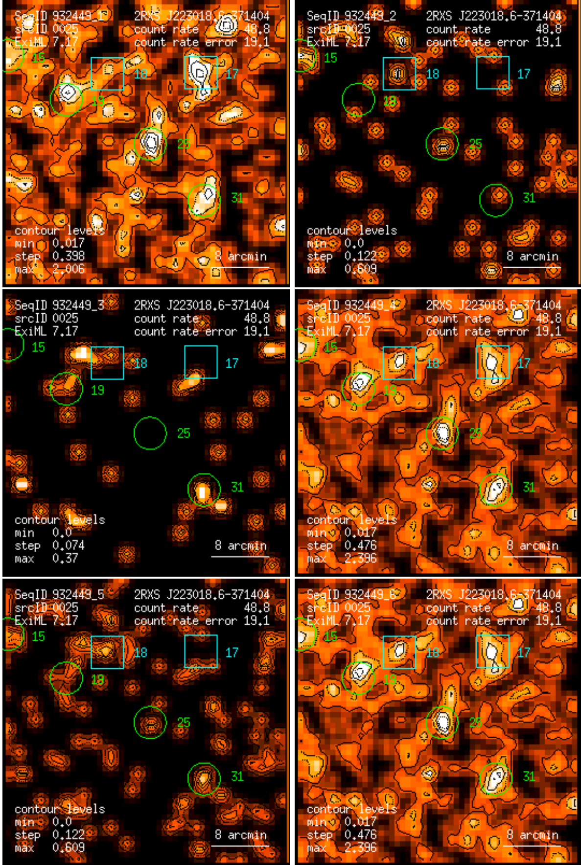
Figure 25: RASS 932449: detection 0025: band rate images, Gaussian filter: (1) PSPC channels 11 – 41, (2) 52 – 90, (3) 91 – 201, (4) 11 – 235, (5) 52 – 201, (6) 11 – 201. Broad band rates in counts/ks. Band rate contour levels in counts/ks/arcmin 2 .
