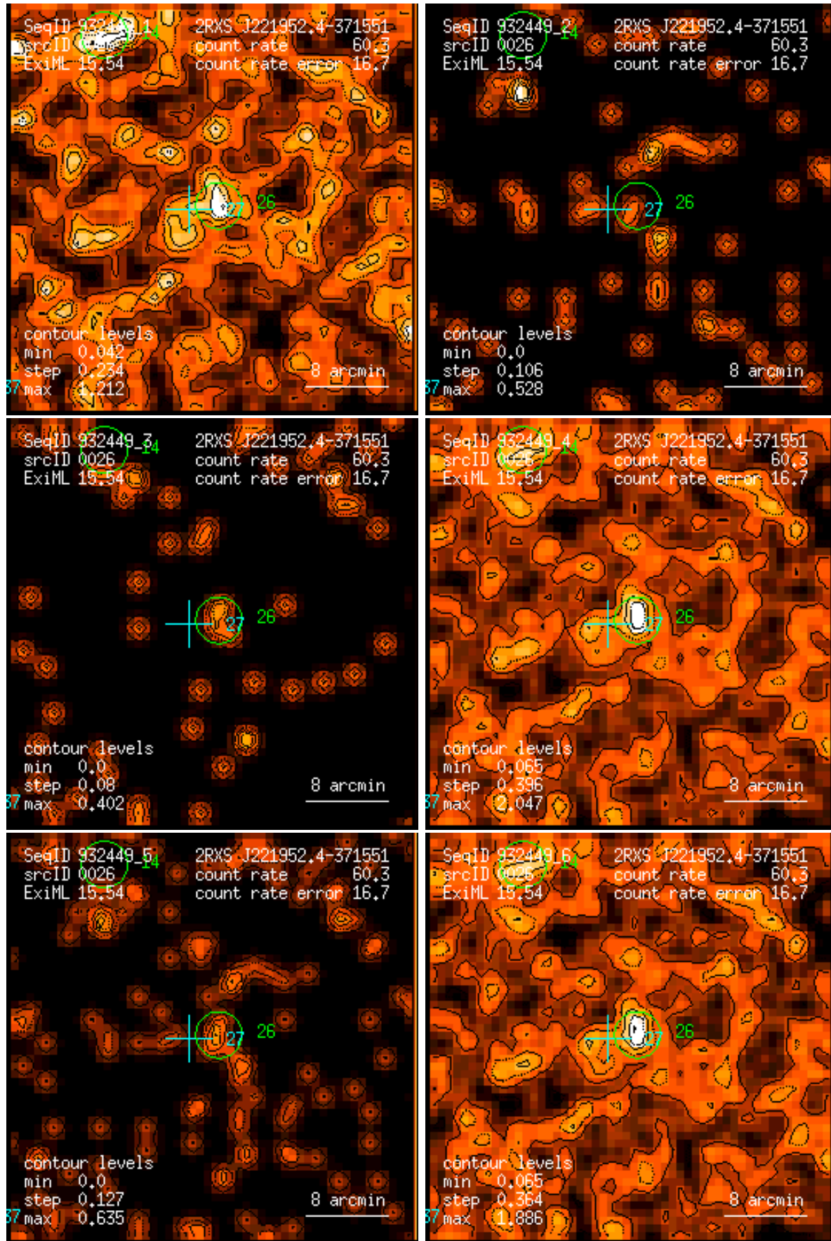
Figure 26: RASS 932449: detection 0026: band rate images, Gaussian filter: (1) PSPC channels 11 – 41, (2) 52 – 90, (3) 91 – 201, (4) 11 – 235, (5) 52 – 201, (6) 11 – 201. Broad band rates in counts/ks. Band rate contour levels in counts/ks/arcmin 2 .
