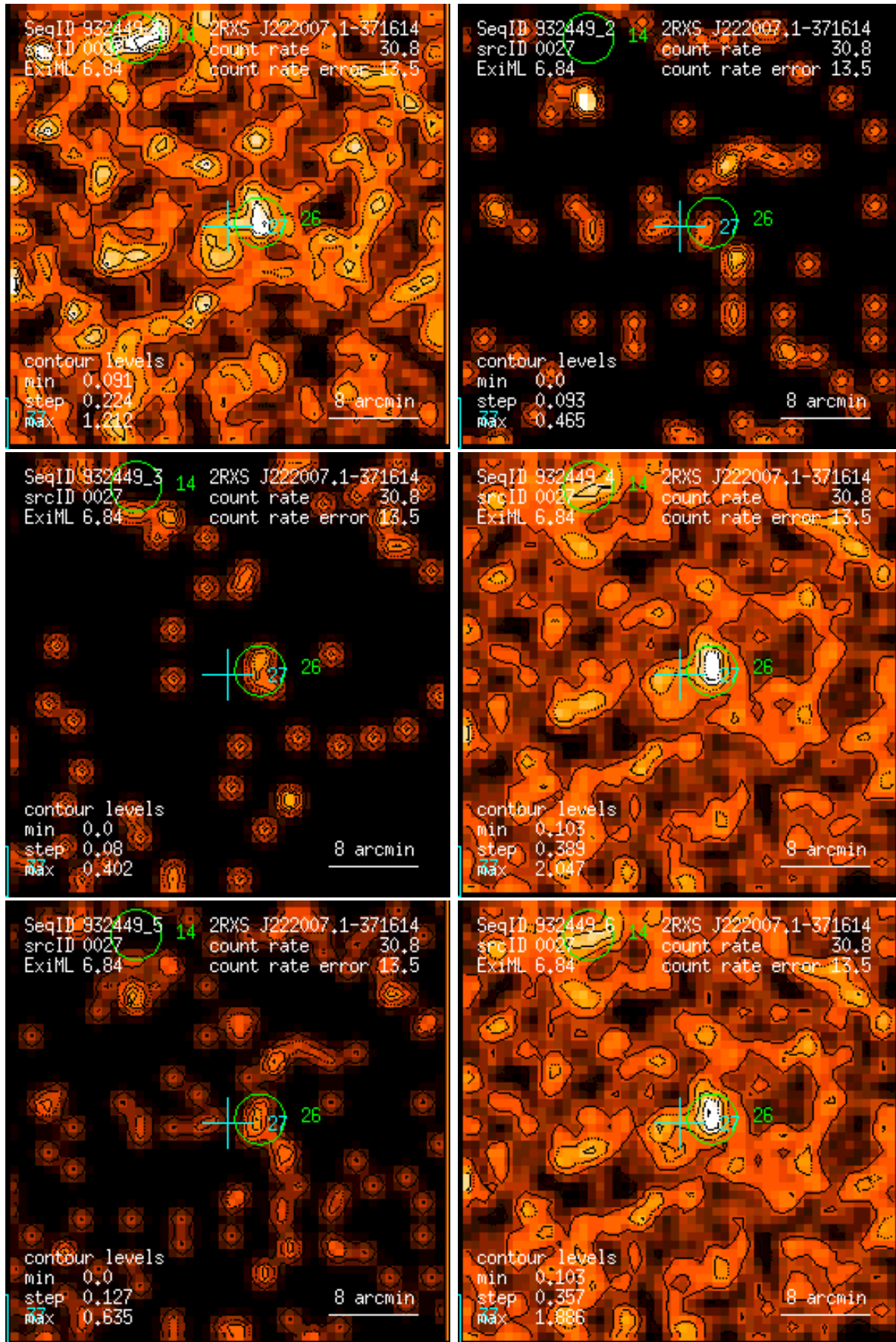
Figure 27: RASS 932449: detection 0027: band rate images, Gaussian filter: (1) PSPC channels 11 – 41, (2) 52 – 90, (3) 91 – 201, (4) 11 – 235, (5) 52 – 201, (6) 11 – 201. Broad band rates in counts/ks. Band rate contour levels in counts/ks/arcmin 2 .
