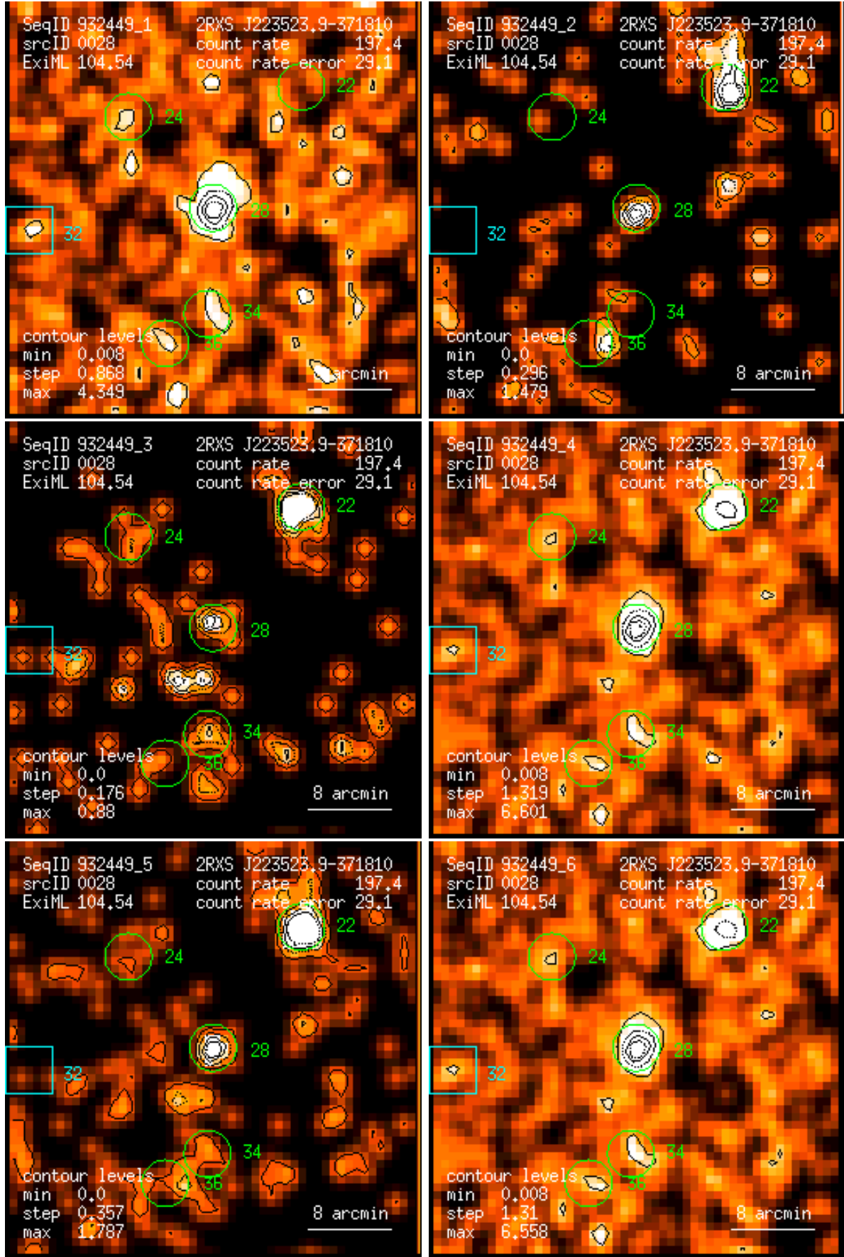
Figure 28: RASS 932449: detection 0028: band rate images, Gaussian filter: (1) PSPC channels 11 – 41, (2) 52 – 90, (3) 91 – 201, (4) 11 – 235, (5) 52 – 201, (6) 11 – 201. Broad band rates in counts/ks. Band rate contour levels in counts/ks/arcmin 2 .
