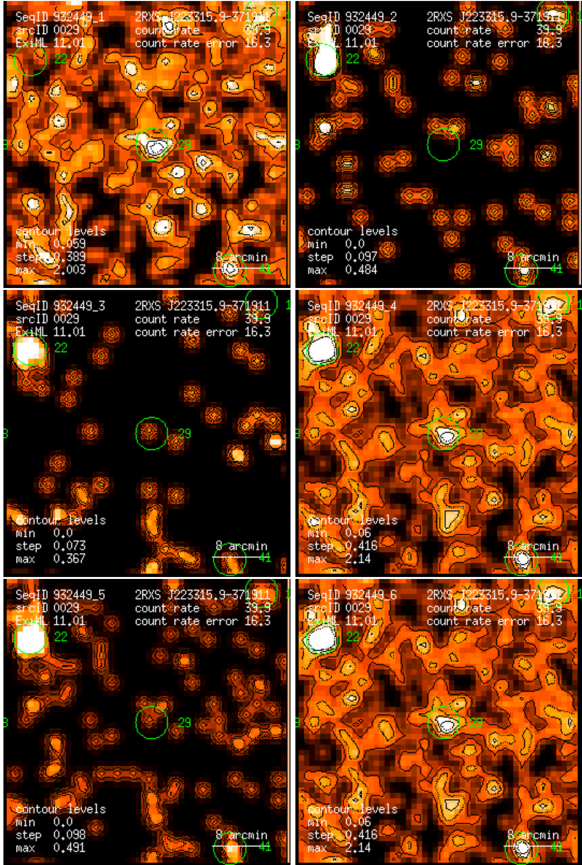
Figure 29: RASS 932449: detection 0029: band rate images, Gaussian filter: (1) PSPC channels 11 – 41, (2) 52 – 90, (3) 91 – 201, (4) 11 – 235, (5) 52 – 201, (6) 11 – 201. Broad band rates in counts/ks. Band rate contour levels in counts/ks/arcmin 2 .
