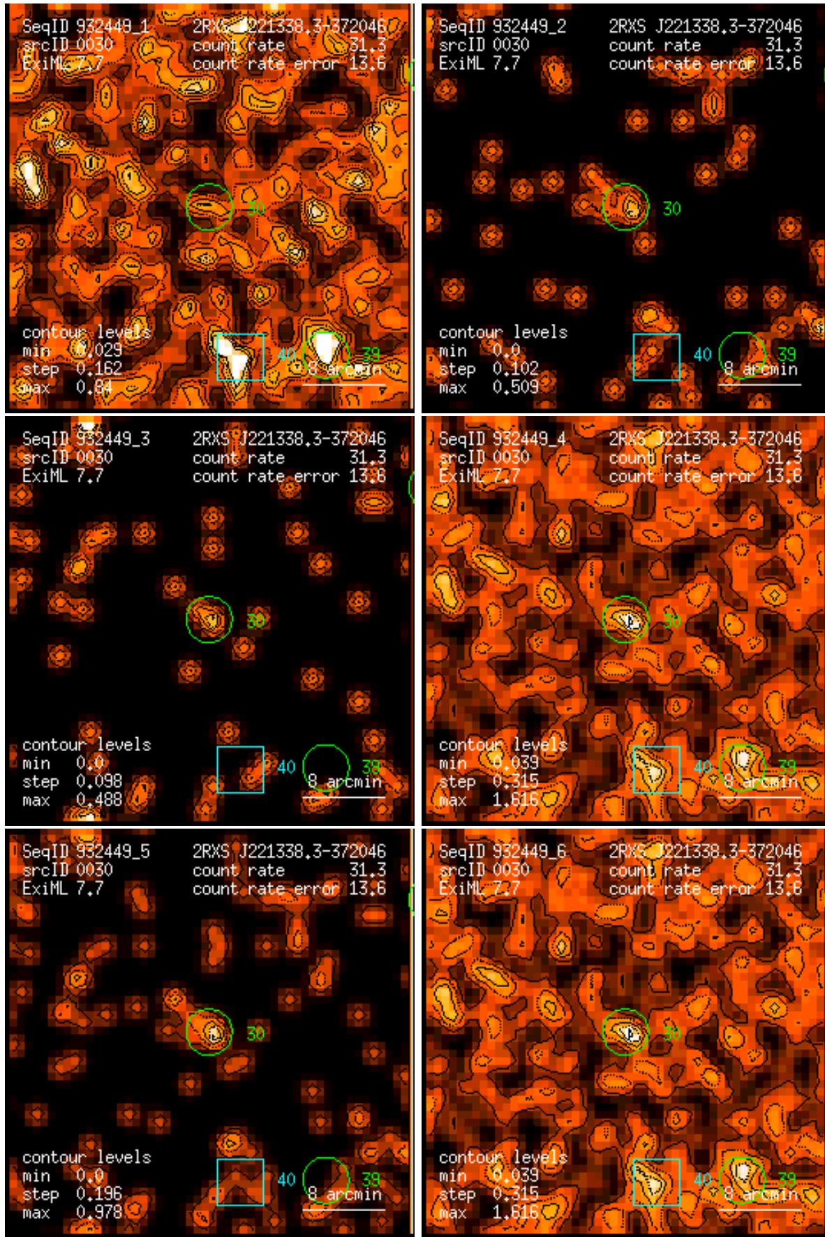
Figure 30: RASS 932449: detection 0030: band rate images, Gaussian filter: (1) PSPC channels 11 – 41, (2) 52 – 90, (3) 91 – 201, (4) 11 – 235, (5) 52 – 201, (6) 11 – 201. Broad band rates in counts/ks. Band rate contour levels in counts/ks/arcmin 2 .
