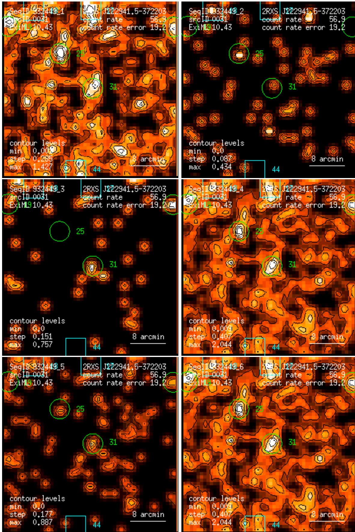
Figure 31: RASS 932449: detection 0031: band rate images, Gaussian filter: (1) PSPC channels 11 – 41, (2) 52 – 90, (3) 91 – 201, (4) 11 – 235, (5) 52 – 201, (6) 11 – 201. Broad band rates in counts/ks. Band rate contour levels in counts/ks/arcmin 2 .
