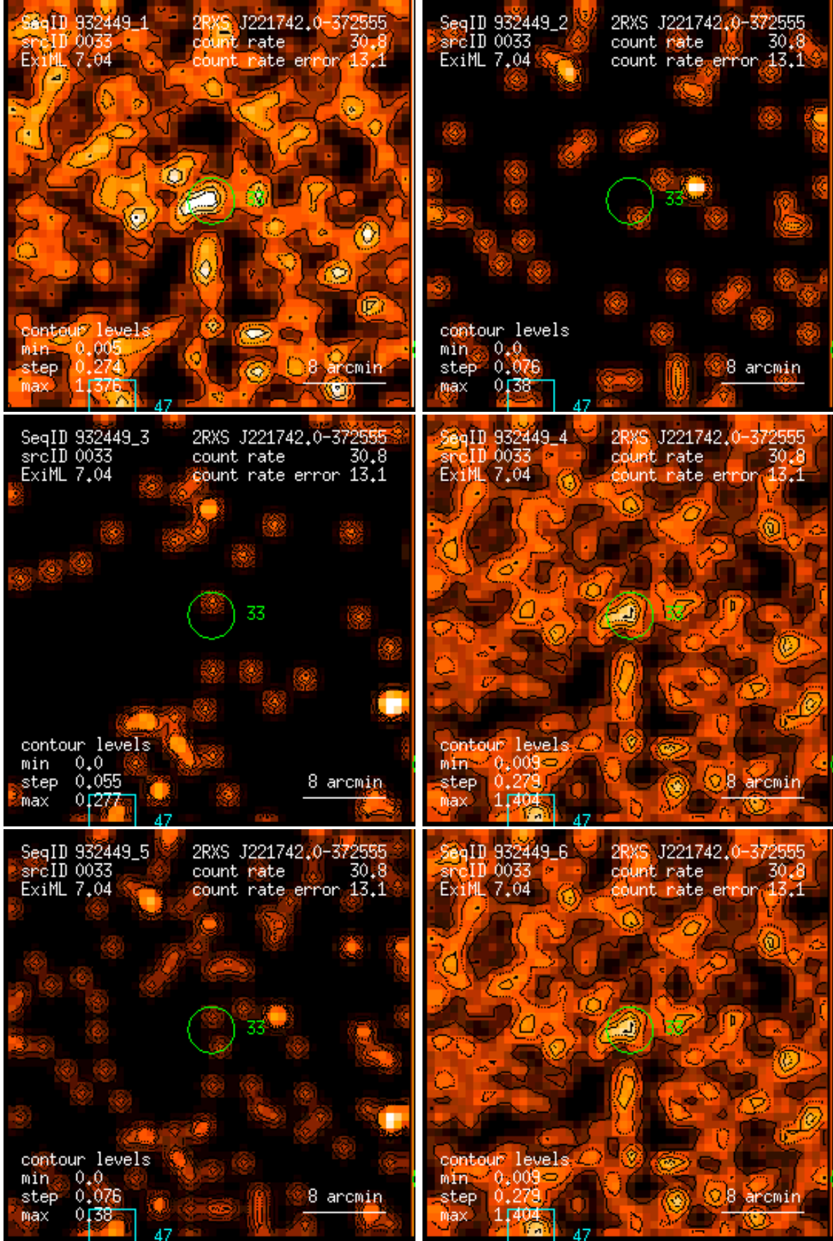
Figure 33: RASS 932449: detection 0033: band rate images, Gaussian filter: (1) PSPC channels 11 – 41, (2) 52 – 90, (3) 91 – 201, (4) 11 – 235, (5) 52 – 201, (6) 11 – 201. Broad band rates in counts/ks. Band rate contour levels in counts/ks/arcmin 2 .
