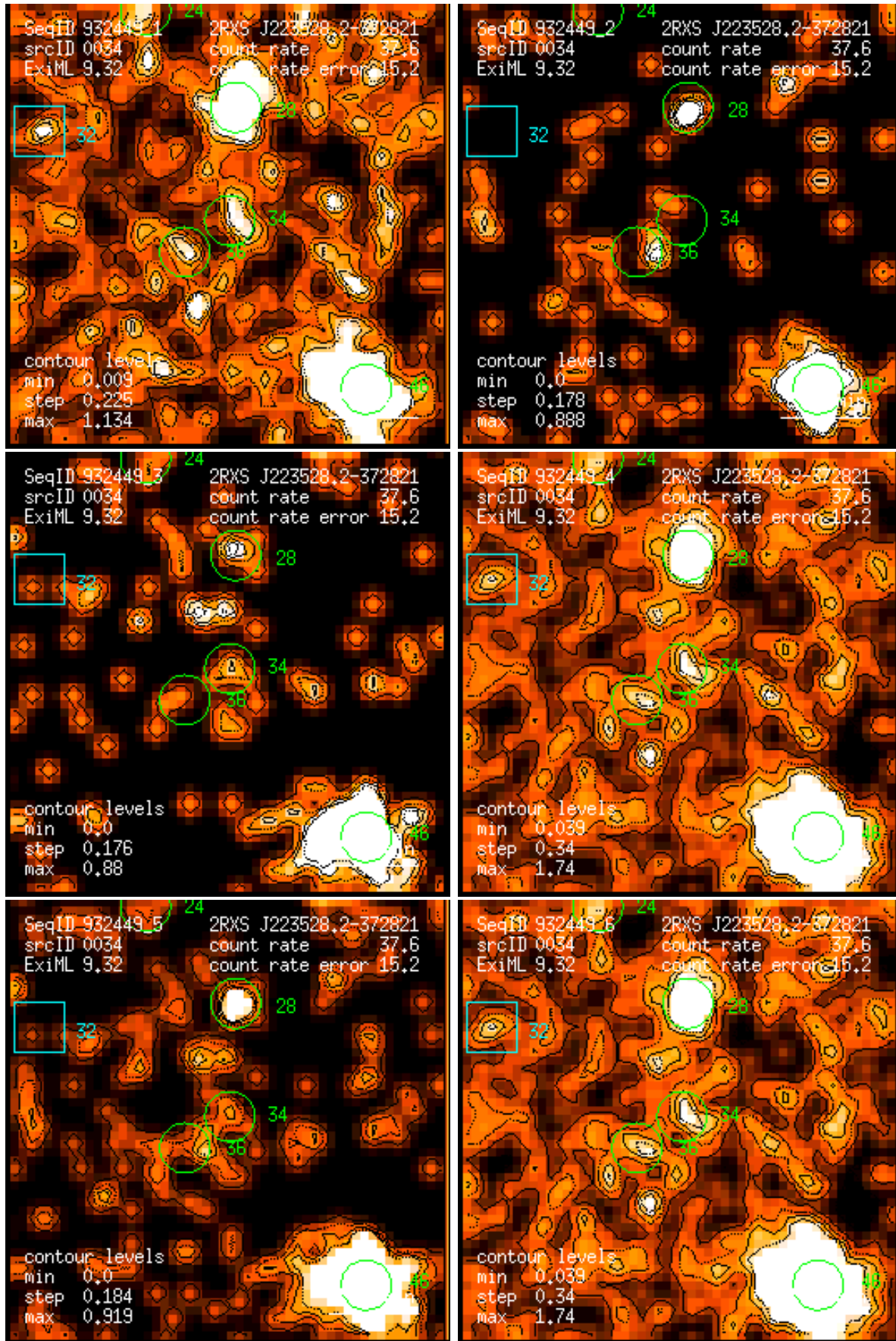
Figure 34: RASS 932449: detection 0034: band rate images, Gaussian filter: (1) PSPC channels 11 – 41, (2) 52 – 90, (3) 91 – 201, (4) 11 – 235, (5) 52 – 201, (6) 11 – 201. Broad band rates in counts/ks. Band rate contour levels in counts/ks/arcmin 2 .
