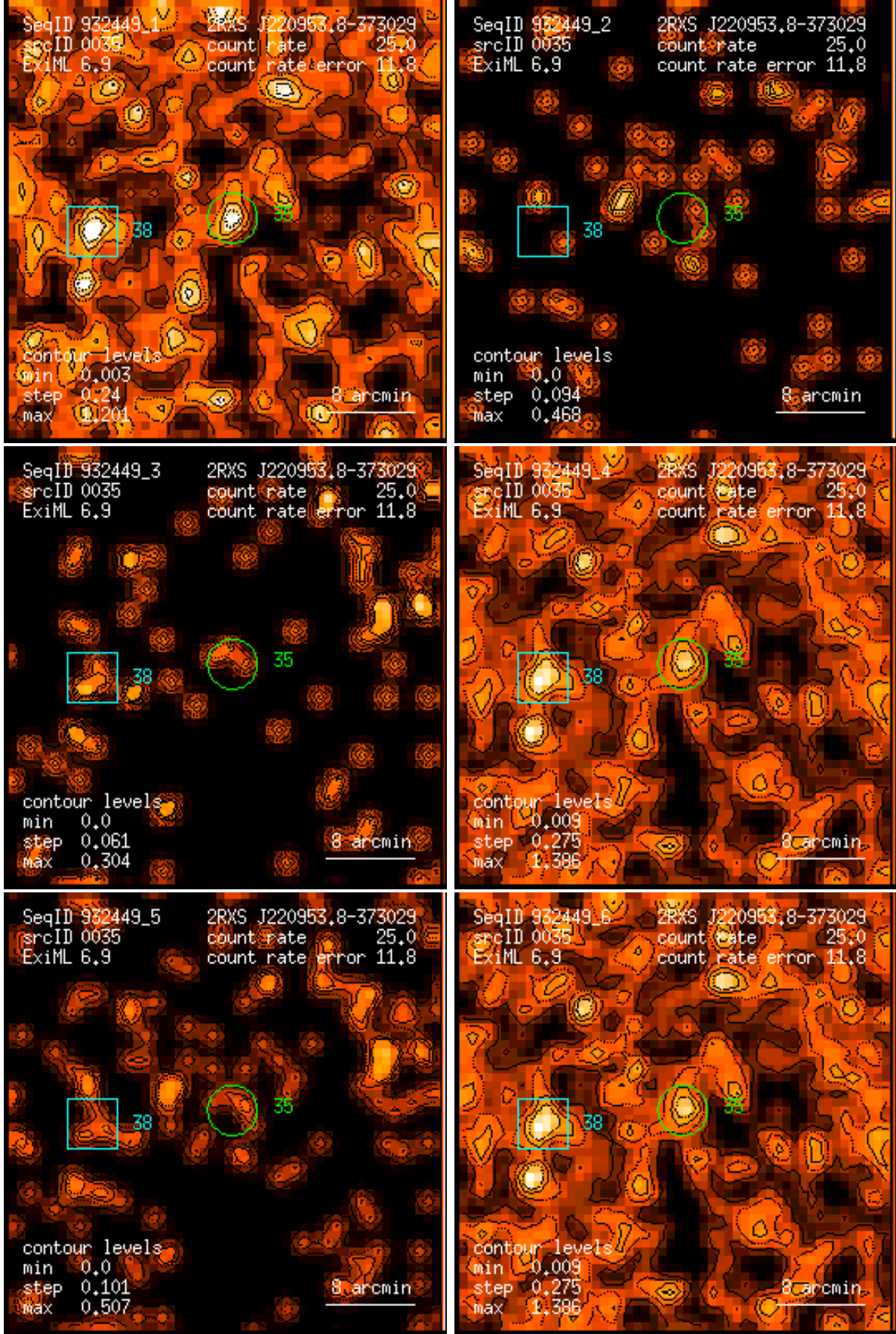
Figure 35: RASS 932449: detection 0035: band rate images, Gaussian filter: (1) PSPC channels 11 – 41, (2) 52 – 90, (3) 91 – 201, (4) 11 – 235, (5) 52 – 201, (6) 11 – 201. Broad band rates in counts/ks. Band rate contour levels in counts/ks/arcmin 2 .
