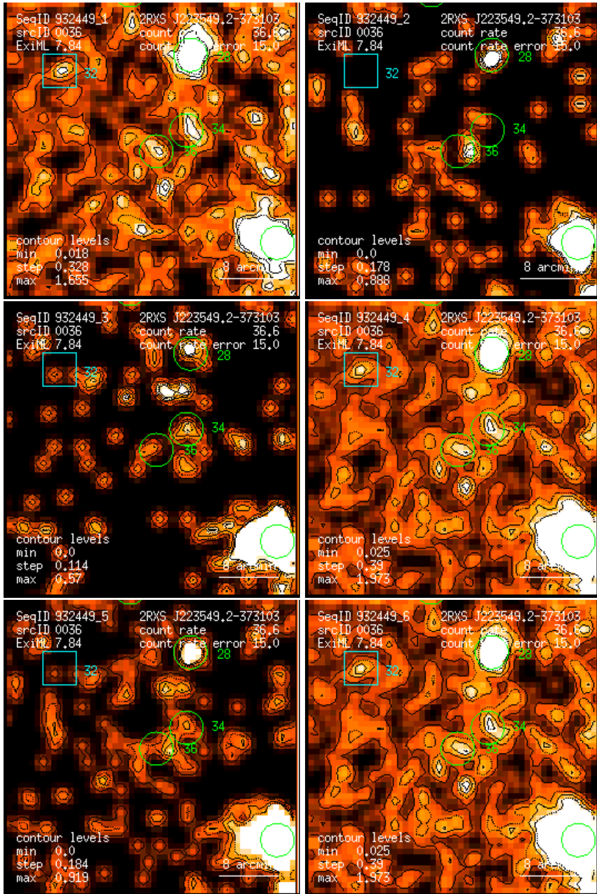
Figure 36: RASS 932449: detection 0036: band rate images, Gaussian filter: (1) PSPC channels 11 – 41, (2) 52 – 90, (3) 91 – 201, (4) 11 – 235, (5) 52 – 201, (6) 11 – 201. Broad band rates in counts/ks. Band rate contour levels in counts/ks/arcmin 2 .
