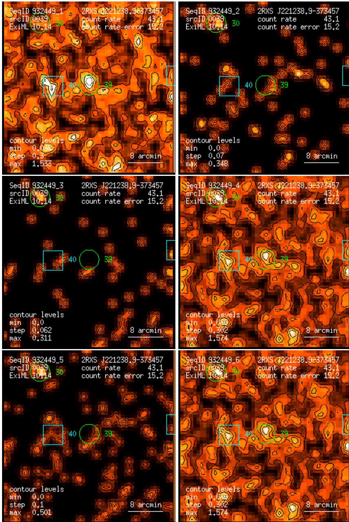
Figure 39: RASS 932449: detection 0039: band rate images, Gaussian filter: (1) PSPC channels 11 – 41, (2) 52 – 90, (3) 91 – 201, (4) 11 – 235, (5) 52 – 201, (6) 11 – 201. Broad band rates in counts/ks. Band rate contour levels in counts/ks/arcmin 2 .
