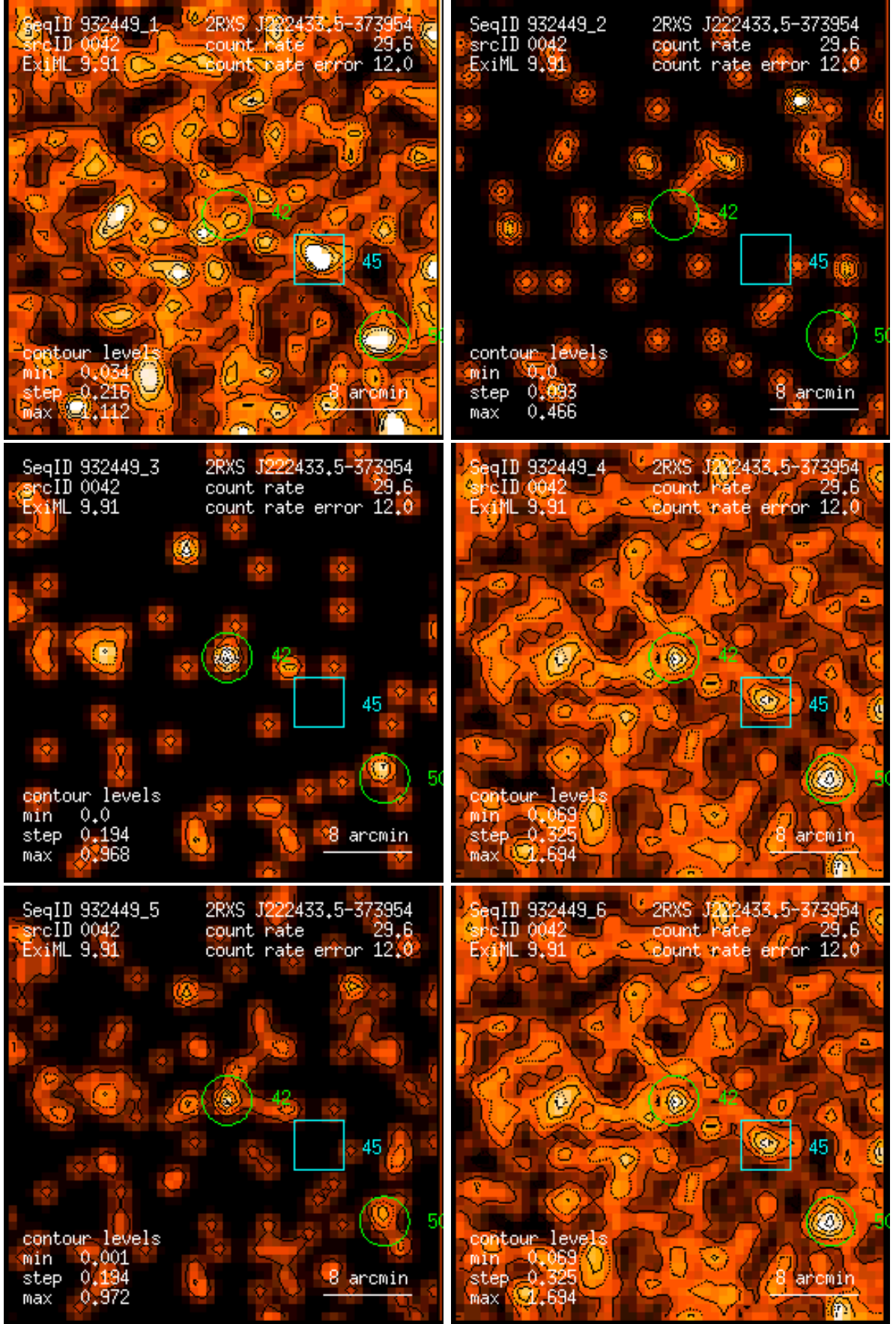
Figure 42: RASS 932449: detection 0042: band rate images, Gaussian filter: (1) PSPC channels 11 – 41, (2) 52 – 90, (3) 91 – 201, (4) 11 – 235, (5) 52 – 201, (6) 11 – 201. Broad band rates in counts/ks. Band rate contour levels in counts/ks/arcmin 2 .
