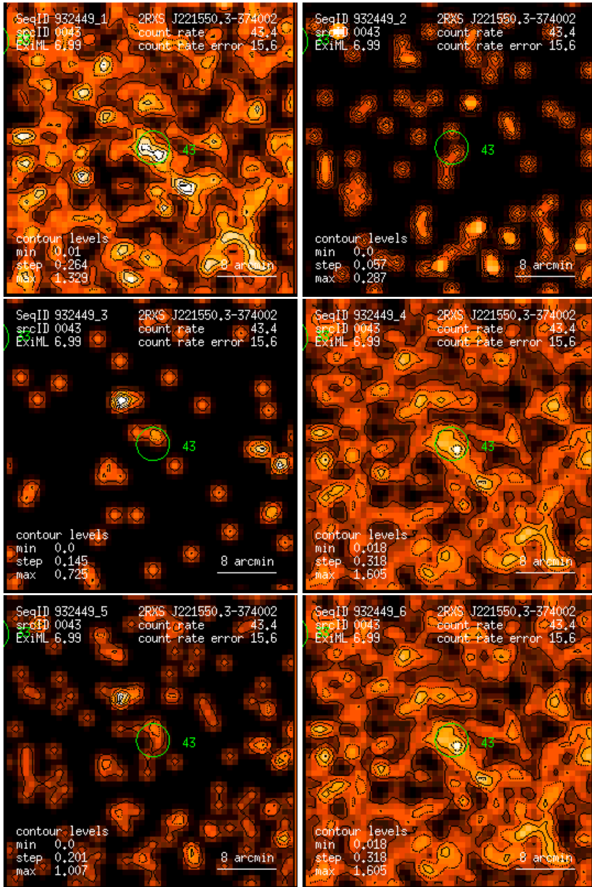
Figure 43: RASS 932449: detection 0043: band rate images, Gaussian filter: (1) PSPC channels 11 – 41, (2) 52 – 90, (3) 91 – 201, (4) 11 – 235, (5) 52 – 201, (6) 11 – 201. Broad band rates in counts/ks. Band rate contour levels in counts/ks/arcmin 2 .
