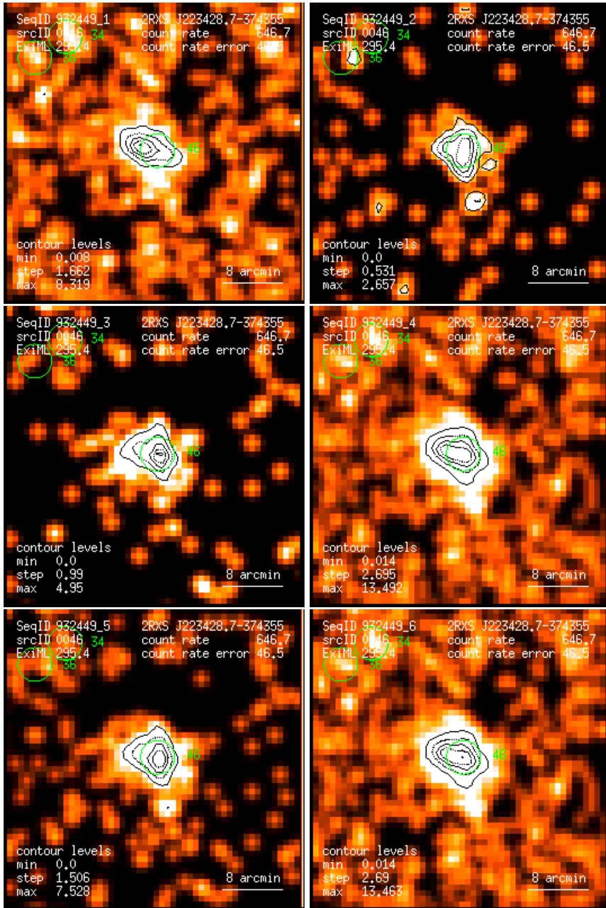
Figure 46: RASS 932449: detection 0046: band rate images, Gaussian filter: (1) PSPC channels 11 – 41, (2) 52 – 90, (3) 91 – 201, (4) 11 – 235, (5) 52 – 201, (6) 11 – 201. Broad band rates in counts/ks. Band rate contour levels in counts/ks/arcmin 2 .
