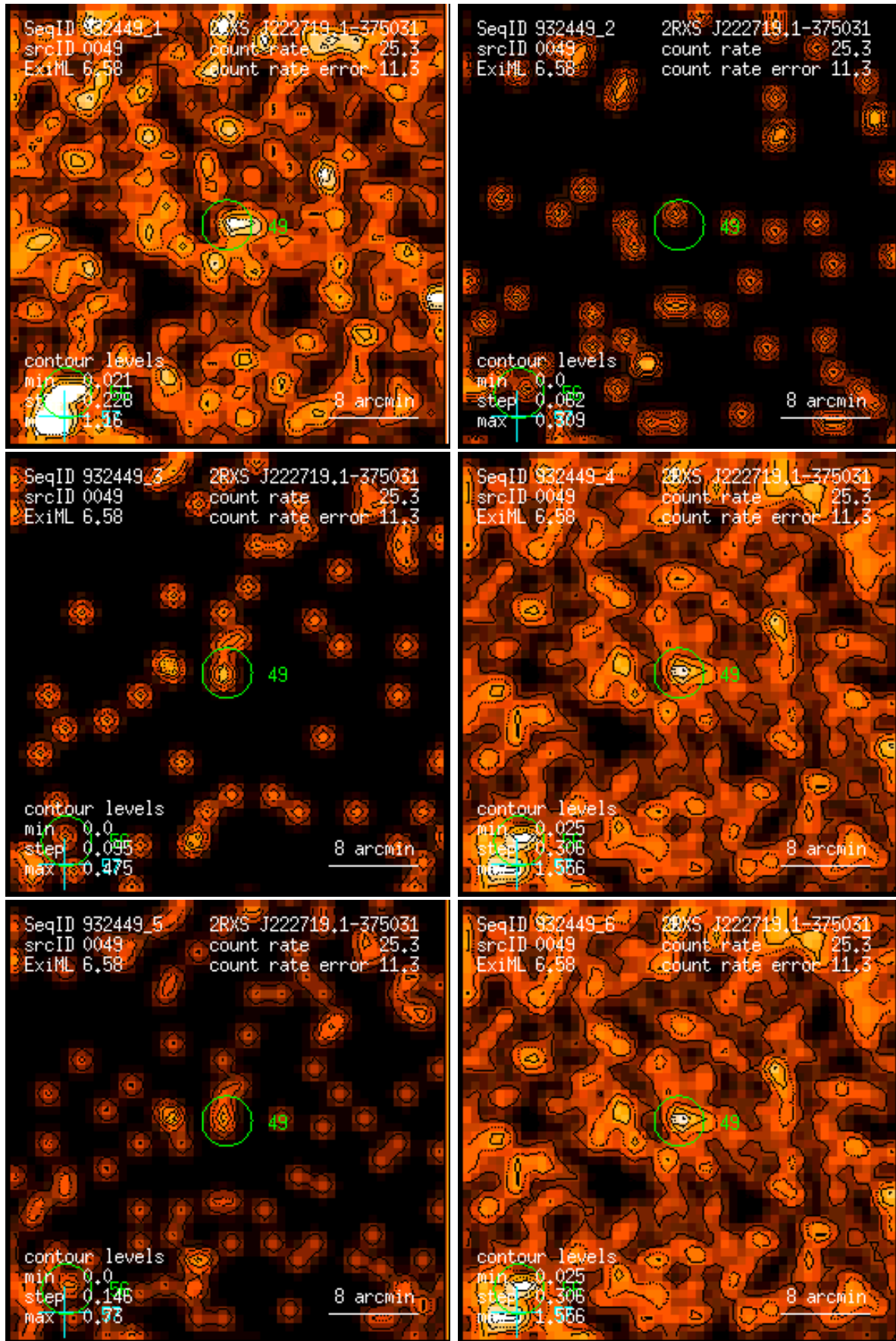
Figure 49: RASS 932449: detection 0049: band rate images, Gaussian filter: (1) PSPC channels 11 – 41, (2) 52 – 90, (3) 91 – 201, (4) 11 – 235, (5) 52 – 201, (6) 11 – 201. Broad band rates in counts/ks. Band rate contour levels in counts/ks/arcmin 2 .
