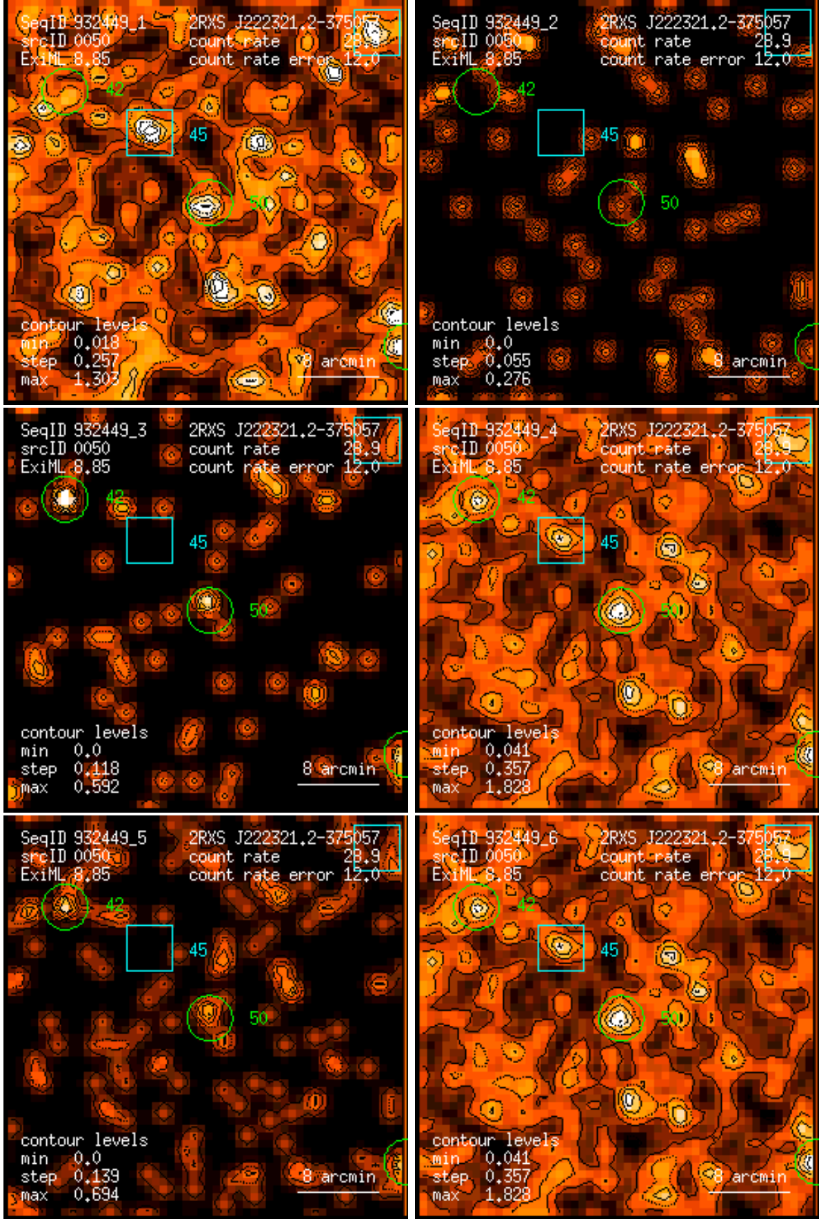
Figure 50: RASS 932449: detection 0050: band rate images, Gaussian filter: (1) PSPC channels 11 – 41, (2) 52 – 90, (3) 91 – 201, (4) 11 – 235, (5) 52 – 201, (6) 11 – 201. Broad band rates in counts/ks. Band rate contour levels in counts/ks/arcmin 2 .
