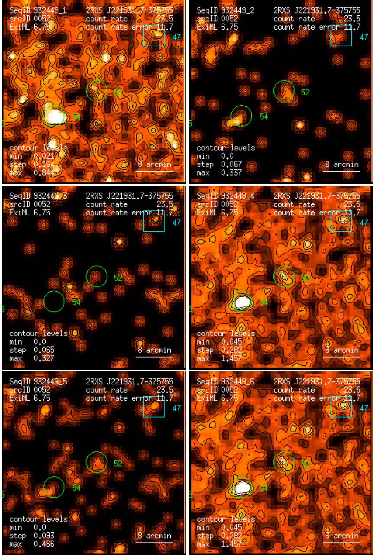
Figure 52: RASS 932449: detection 0052: band rate images, Gaussian filter: (1) PSPC channels 11 – 41, (2) 52 – 90, (3) 91 – 201, (4) 11 – 235, (5) 52 – 201, (6) 11 – 201. Broad band rates in counts/ks. Band rate contour levels in counts/ks/arcmin 2 .
