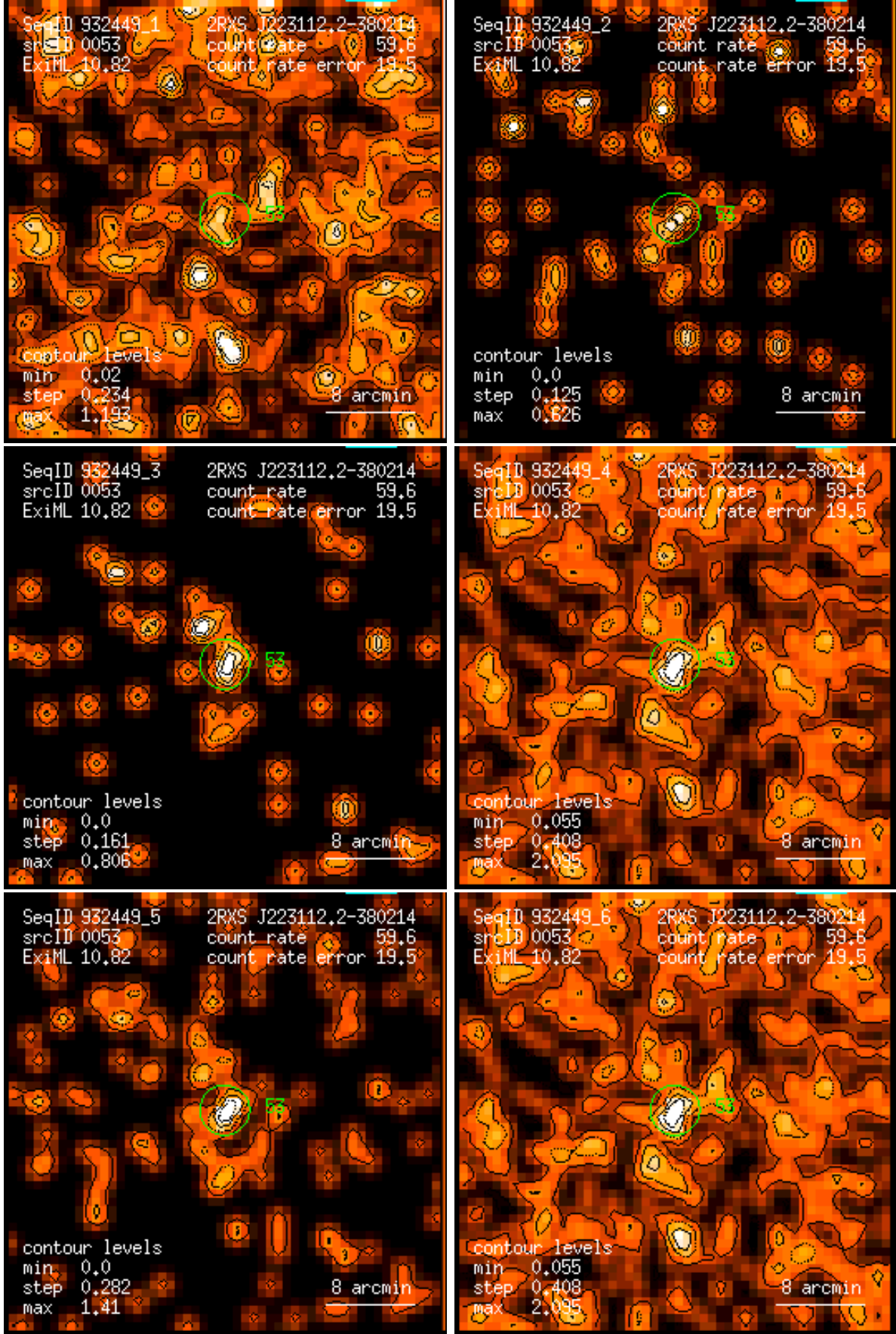
Figure 53: RASS 932449: detection 0053: band rate images, Gaussian filter: (1) PSPC channels 11 – 41, (2) 52 – 90, (3) 91 – 201, (4) 11 – 235, (5) 52 – 201, (6) 11 – 201. Broad band rates in counts/ks. Band rate contour levels in counts/ks/arcmin 2 .
