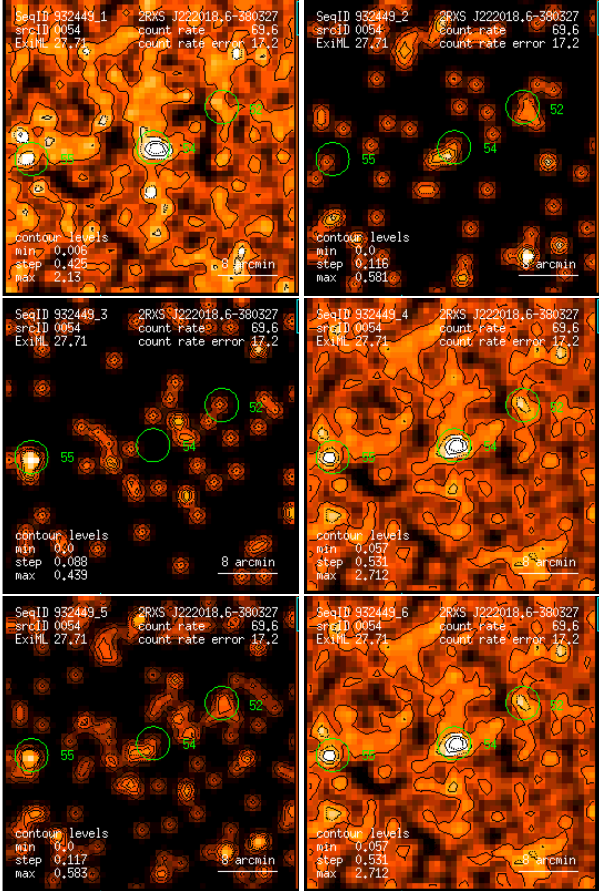
Figure 54: RASS 932449: detection 0054: band rate images, Gaussian filter: (1) PSPC channels 11 – 41, (2) 52 – 90, (3) 91 – 201, (4) 11 – 235, (5) 52 – 201, (6) 11 – 201. Broad band rates in counts/ks. Band rate contour levels in counts/ks/arcmin 2 .
