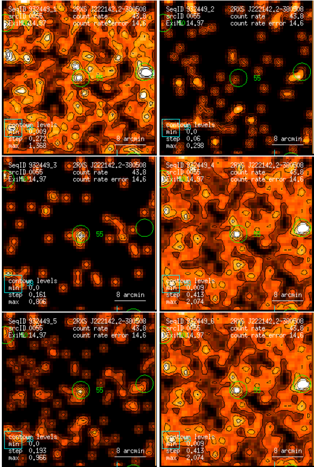
Figure 55: RASS 932449: detection 0055: band rate images, Gaussian filter: (1) PSPC channels 11 – 41, (2) 52 – 90, (3) 91 – 201, (4) 11 – 235, (5) 52 – 201, (6) 11 – 201. Broad band rates in counts/ks. Band rate contour levels in counts/ks/arcmin 2 .
