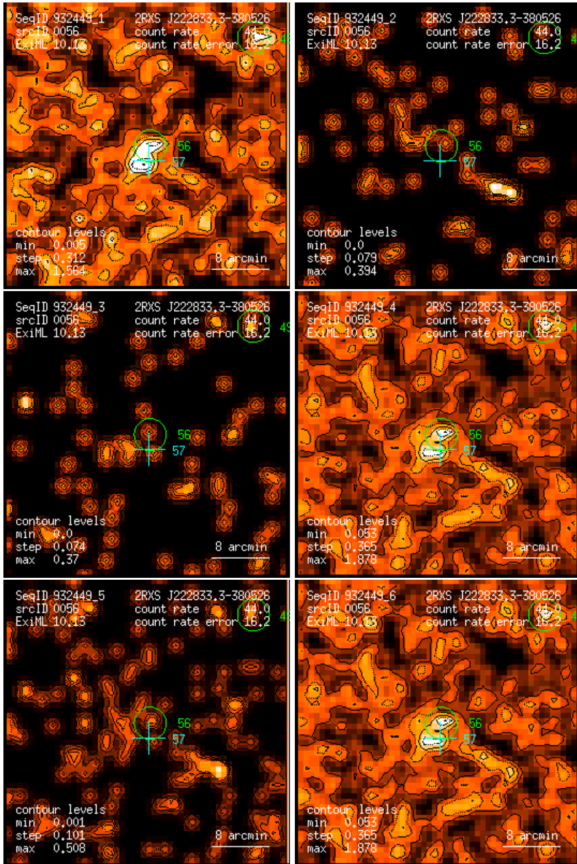
Figure 56: RASS 932449: detection 0056: band rate images, Gaussian filter: (1) PSPC channels 11 – 41, (2) 52 – 90, (3) 91 – 201, (4) 11 – 235, (5) 52 – 201, (6) 11 – 201. Broad band rates in counts/ks. Band rate contour levels in counts/ks/arcmin 2 .
