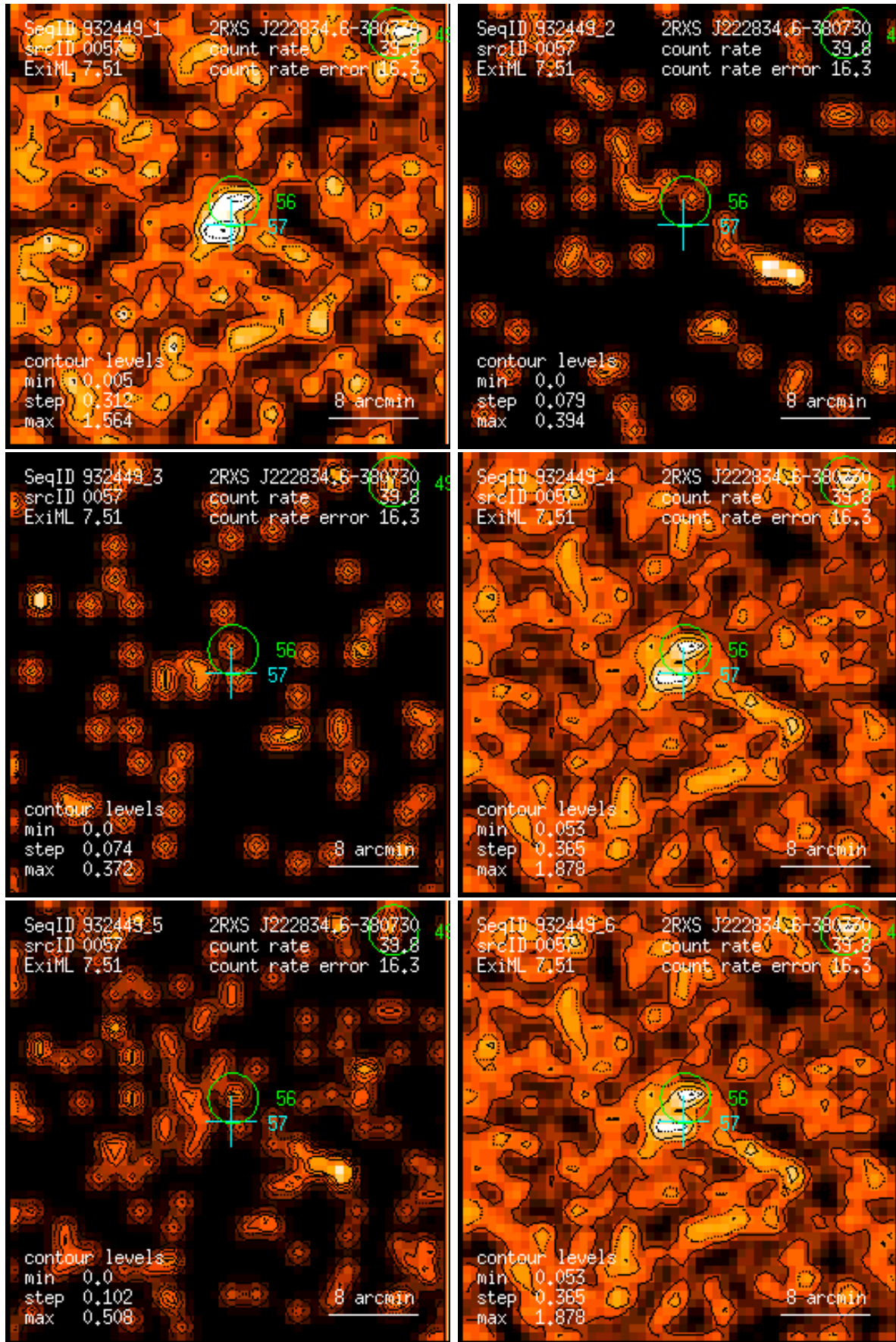
Figure 57: RASS 932449: detection 0057: band rate images, Gaussian filter: (1) PSPC channels 11 – 41, (2) 52 – 90, (3) 91 – 201, (4) 11 – 235, (5) 52 – 201, (6) 11 – 201. Broad band rates in counts/ks. Band rate contour levels in counts/ks/arcmin 2 .
