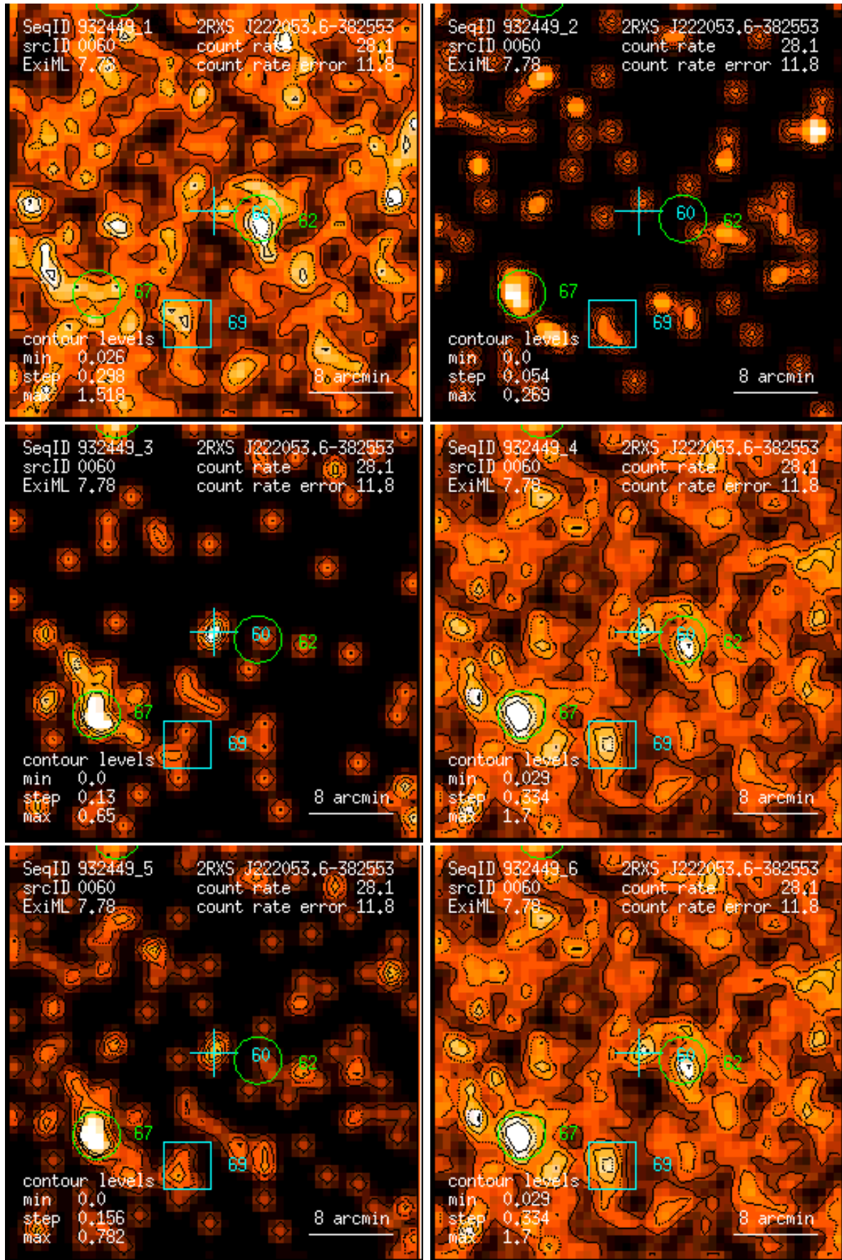
Figure 60: RASS 932449: detection 0060: band rate images, Gaussian filter: (1) PSPC channels 11 – 41, (2) 52 – 90, (3) 91 – 201, (4) 11 – 235, (5) 52 – 201, (6) 11 – 201. Broad band rates in counts/ks. Band rate contour levels in counts/ks/arcmin 2 .
