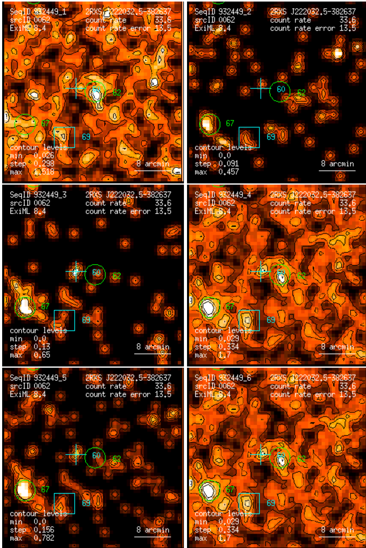
Figure 62: RASS 932449: detection 0062: band rate images, Gaussian filter: (1) PSPC channels 11 – 41, (2) 52 – 90, (3) 91 – 201, (4) 11 – 235, (5) 52 – 201, (6) 11 – 201. Broad band rates in counts/ks. Band rate contour levels in counts/ks/arcmin 2 .
