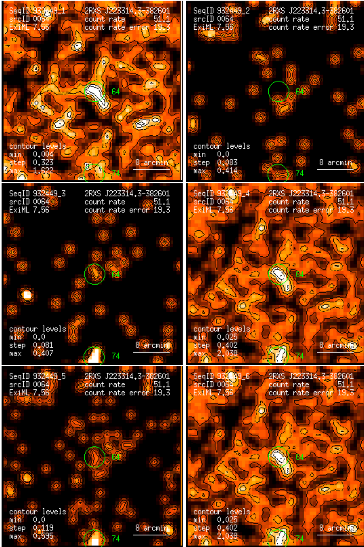
Figure 64: RASS 932449: detection 0064: band rate images, Gaussian filter: (1) PSPC channels 11 – 41, (2) 52 – 90, (3) 91 – 201, (4) 11 – 235, (5) 52 – 201, (6) 11 – 201. Broad band rates in counts/ks. Band rate contour levels in counts/ks/arcmin 2 .
