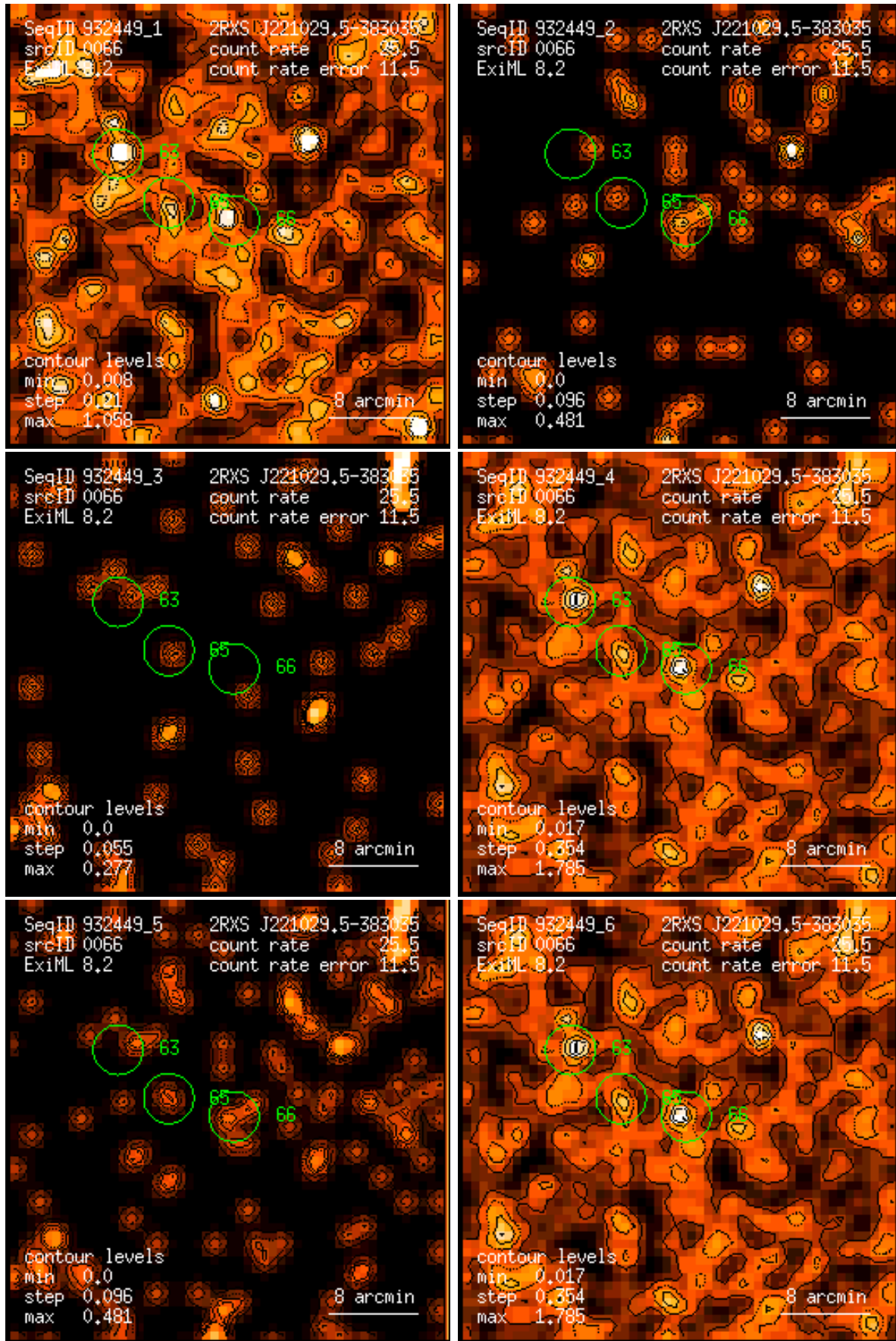
Figure 66: RASS 932449: detection 0066: band rate images, Gaussian filter: (1) PSPC channels 11 – 41, (2) 52 – 90, (3) 91 – 201, (4) 11 – 235, (5) 52 – 201, (6) 11 – 201. Broad band rates in counts/ks. Band rate contour levels in counts/ks/arcmin 2 .
