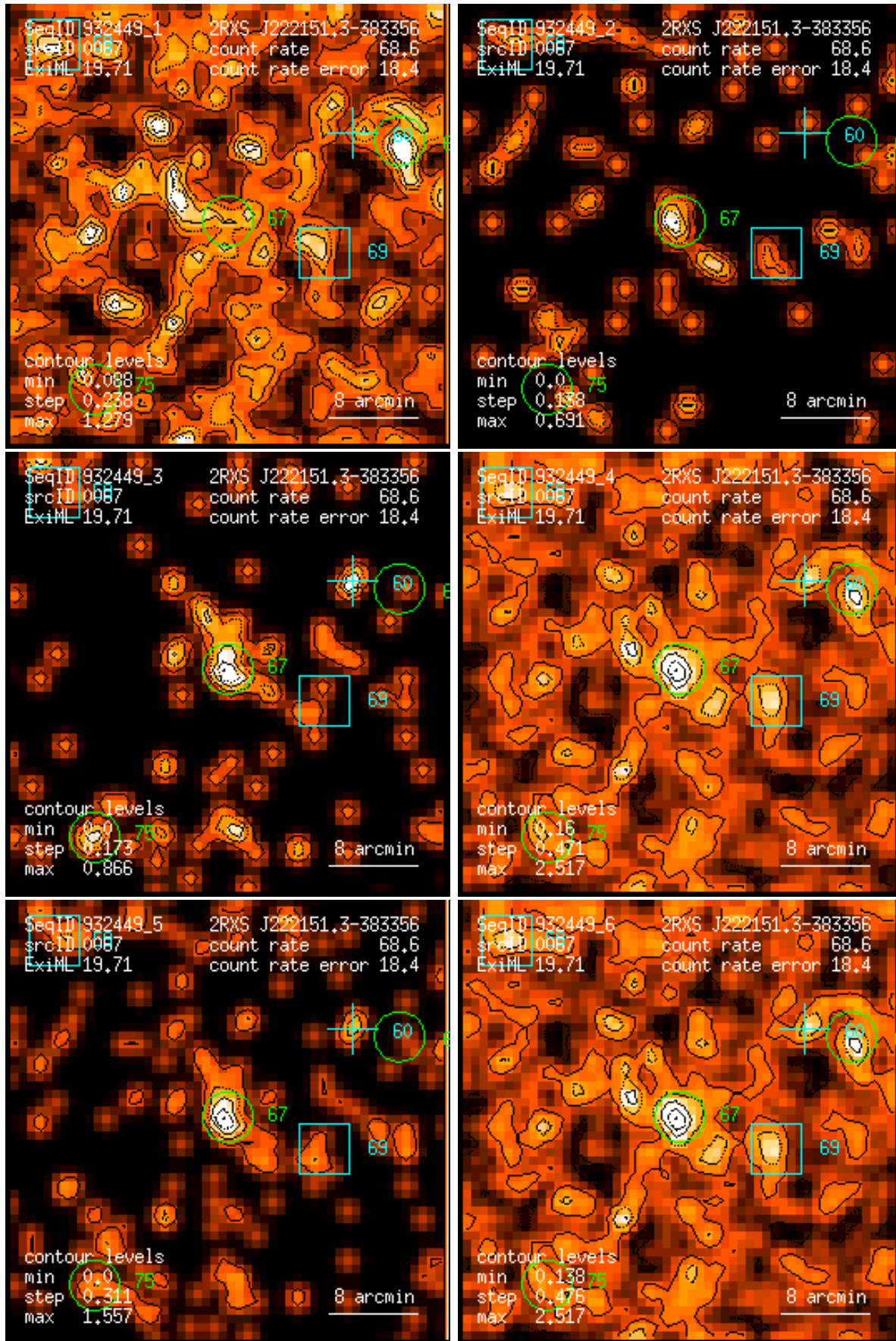
Figure 67: RASS 932449: detection 0067: band rate images, Gaussian filter: (1) PSPC channels 11 – 41, (2) 52 – 90, (3) 91 – 201, (4) 11 – 235, (5) 52 – 201, (6) 11 – 201. Broad band rates in counts/ks. Band rate contour levels in counts/ks/arcmin 2 .
