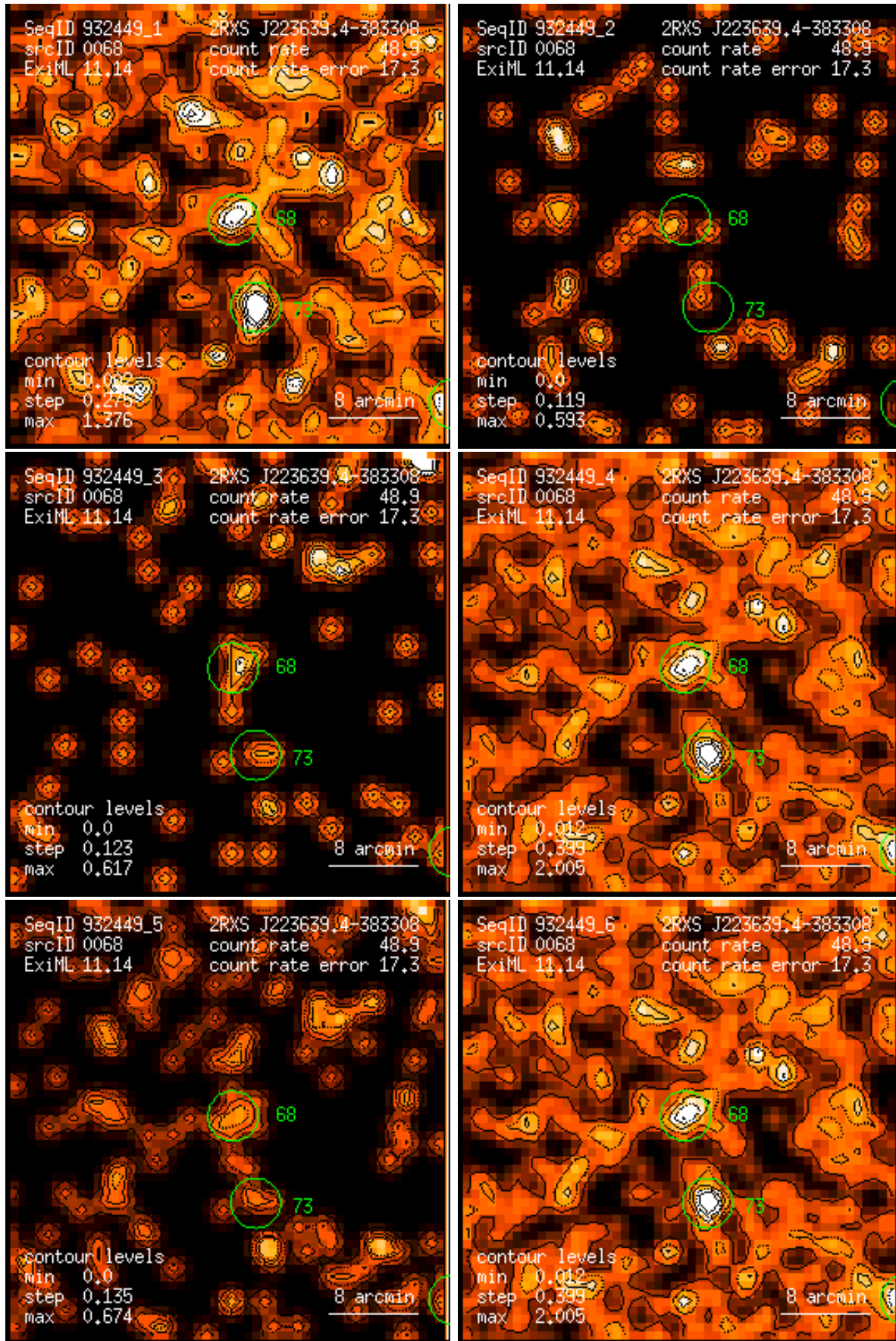
Figure 68: RASS 932449: detection 0068: band rate images, Gaussian filter: (1) PSPC channels 11 – 41, (2) 52 – 90, (3) 91 – 201, (4) 11 – 235, (5) 52 – 201, (6) 11 – 201. Broad band rates in counts/ks. Band rate contour levels in counts/ks/arcmin 2 .
