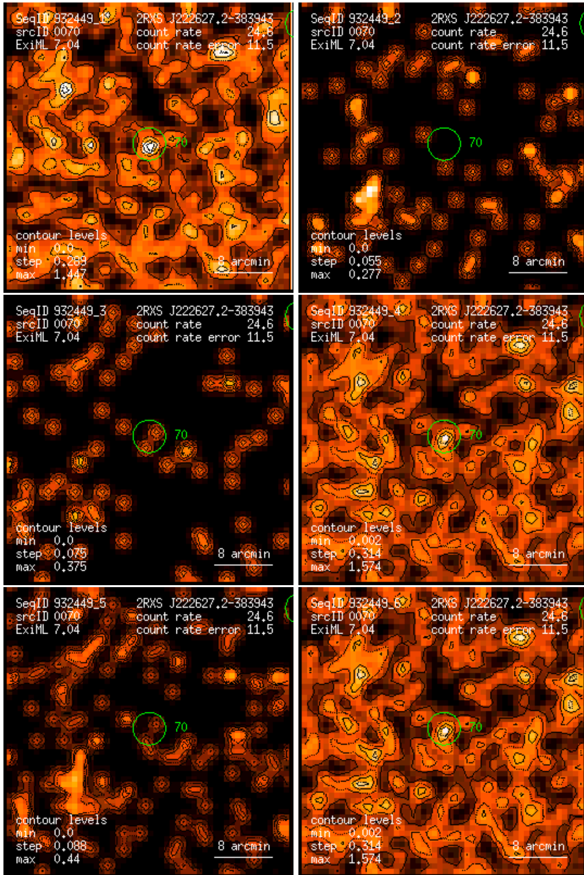
Figure 70: RASS 932449: detection 0070: band rate images, Gaussian filter: (1) PSPC channels 11 – 41, (2) 52 – 90, (3) 91 – 201, (4) 11 – 235, (5) 52 – 201, (6) 11 – 201. Broad band rates in counts/ks. Band rate contour levels in counts/ks/arcmin 2 .
