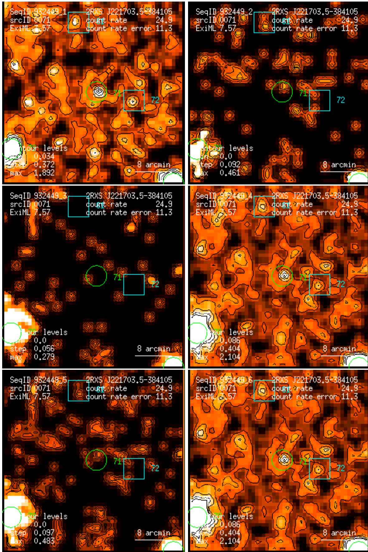
Figure 71: RASS 932449: detection 0071: band rate images, Gaussian filter: (1) PSPC channels 11 – 41, (2) 52 – 90, (3) 91 – 201, (4) 11 – 235, (5) 52 – 201, (6) 11 – 201. Broad band rates in counts/ks. Band rate contour levels in counts/ks/arcmin 2 .
