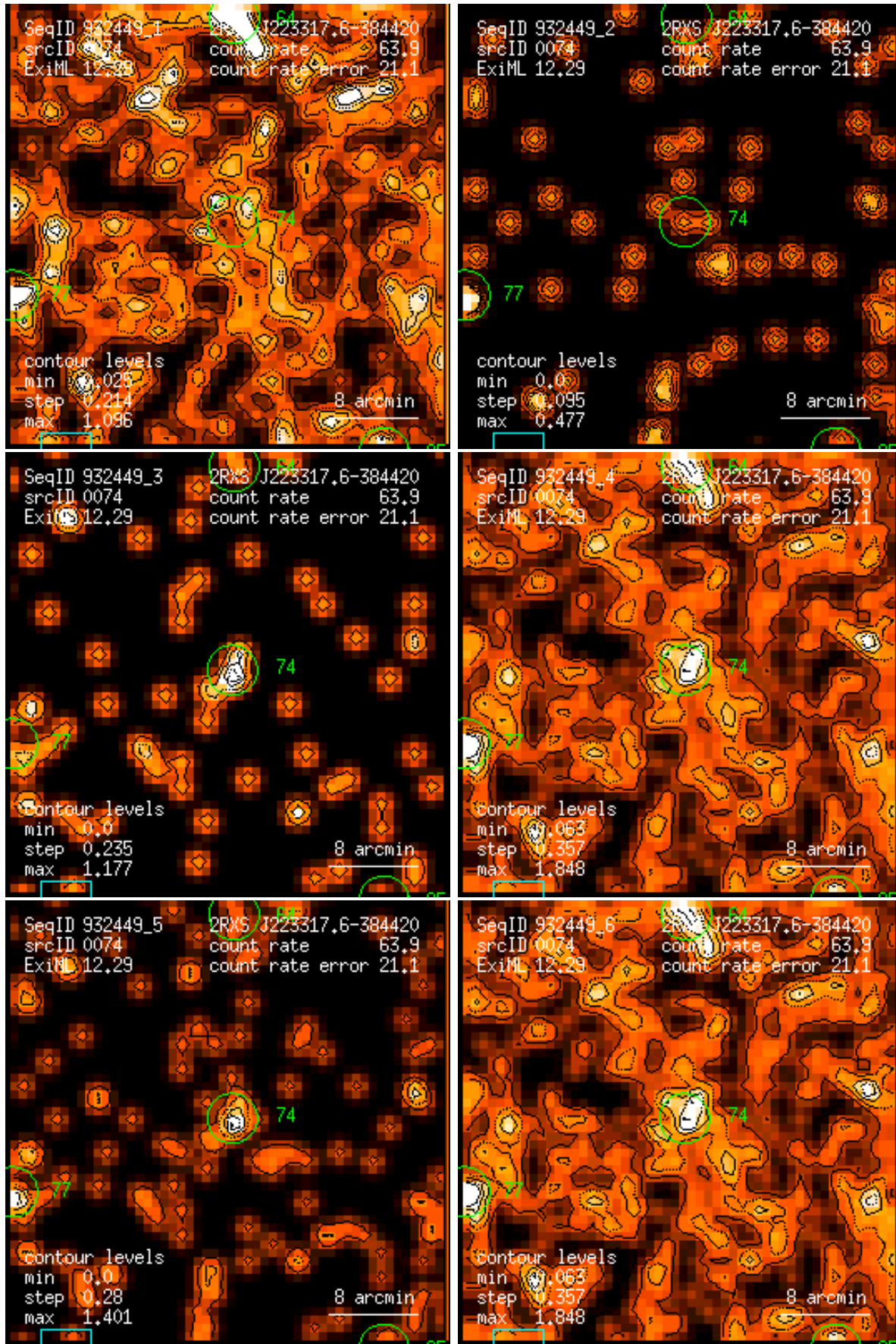
Figure 74: RASS 932449: detection 0074: band rate images, Gaussian filter: (1) PSPC channels 11 – 41, (2) 52 – 90, (3) 91 – 201, (4) 11 – 235, (5) 52 – 201, (6) 11 – 201. Broad band rates in counts/ks. Band rate contour levels in counts/ks/arcmin 2 .
