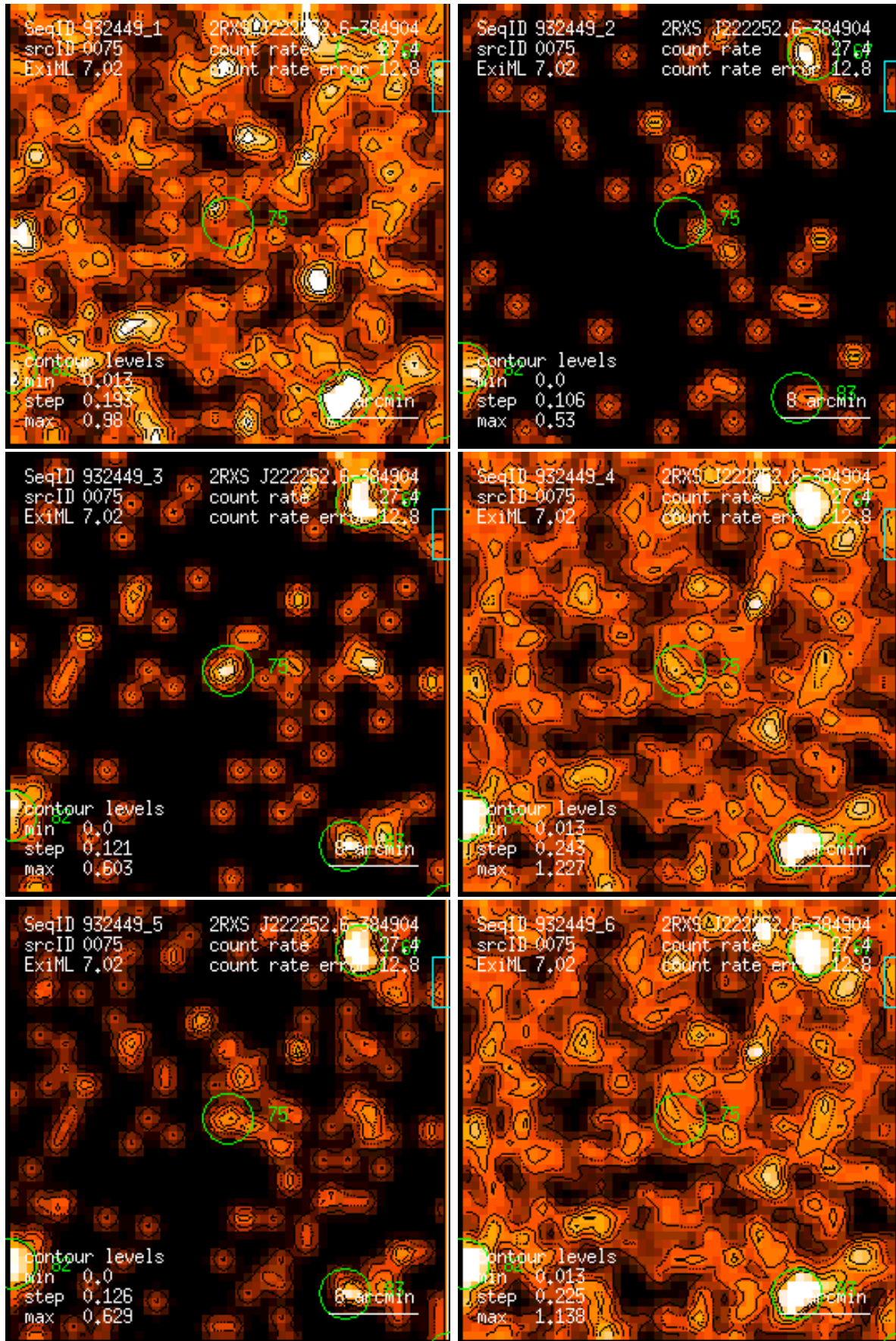
Figure 75: RASS 932449: detection 0075: band rate images, Gaussian filter: (1) PSPC channels 11 – 41, (2) 52 – 90, (3) 91 – 201, (4) 11 – 235, (5) 52 – 201, (6) 11 – 201. Broad band rates in counts/ks. Band rate contour levels in counts/ks/arcmin 2 .
