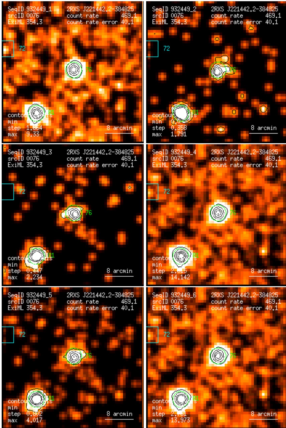
Figure 76: RASS 932449: detection 0076: band rate images, Gaussian filter: (1) PSPC channels 11 – 41, (2) 52 – 90, (3) 91 – 201, (4) 11 – 235, (5) 52 – 201, (6) 11 – 201. Broad band rates in counts/ks. Band rate contour levels in counts/ks/arcmin 2 .
