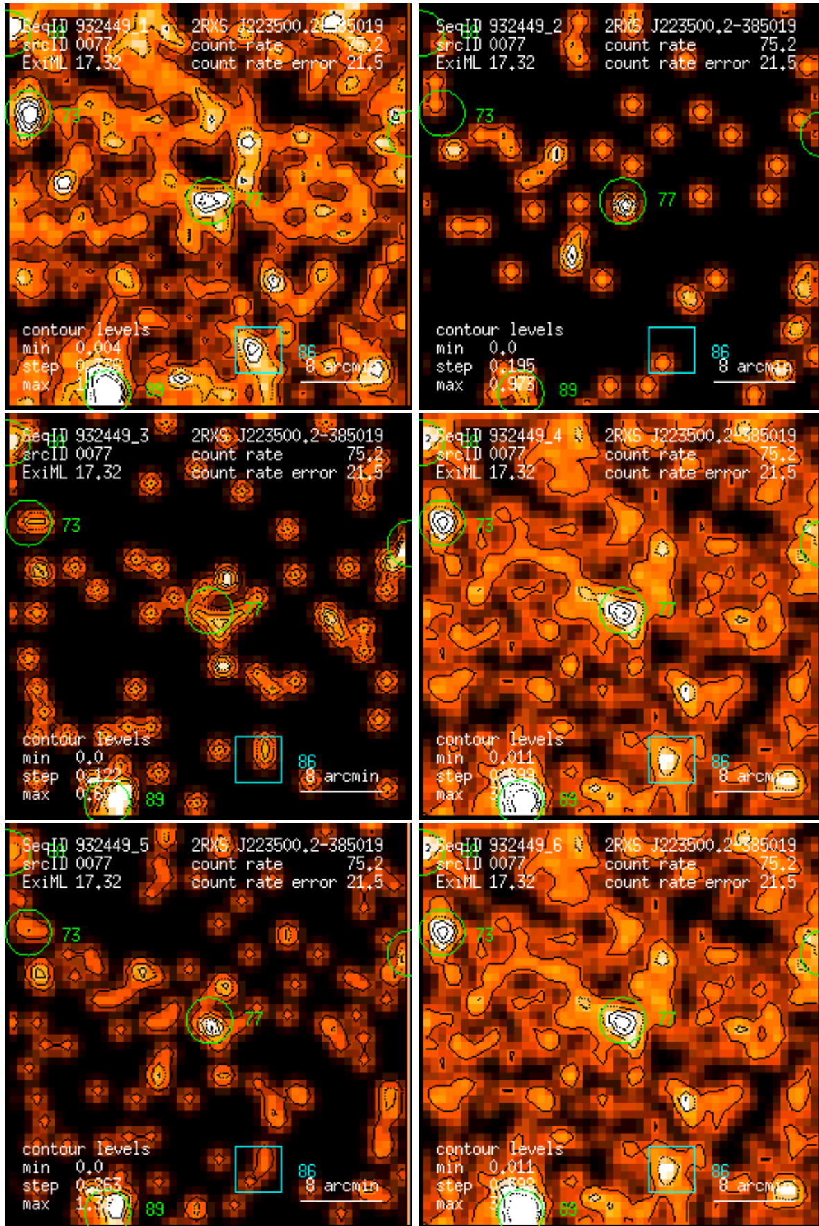
Figure 77: RASS 932449: detection 0077: band rate images, Gaussian filter: (1) PSPC channels 11 – 41, (2) 52 – 90, (3) 91 – 201, (4) 11 – 235, (5) 52 – 201, (6) 11 – 201. Broad band rates in counts/ks. Band rate contour levels in counts/ks/arcmin 2 .
