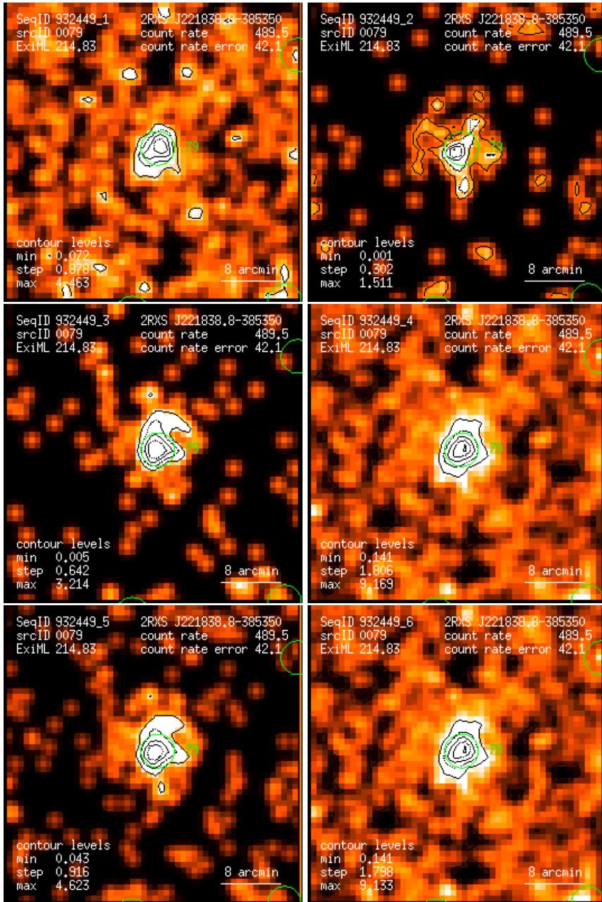
Figure 79: RASS 932449: detection 0079: band rate images, Gaussian filter: (1) PSPC channels 11 – 41, (2) 52 – 90, (3) 91 – 201, (4) 11 – 235, (5) 52 – 201, (6) 11 – 201. Broad band rates in counts/ks. Band rate contour levels in counts/ks/arcmin 2 .
