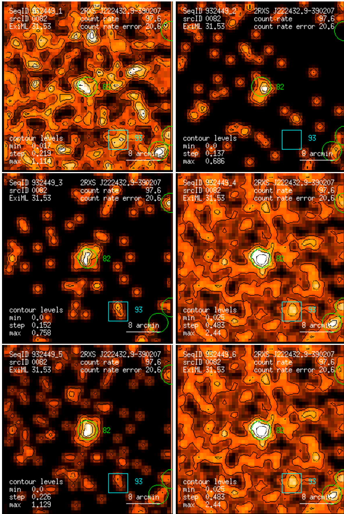
Figure 82: RASS 932449: detection 0082: band rate images, Gaussian filter: (1) PSPC channels 11 – 41, (2) 52 – 90, (3) 91 – 201, (4) 11 – 235, (5) 52 – 201, (6) 11 – 201. Broad band rates in counts/ks. Band rate contour levels in counts/ks/arcmin 2 .
