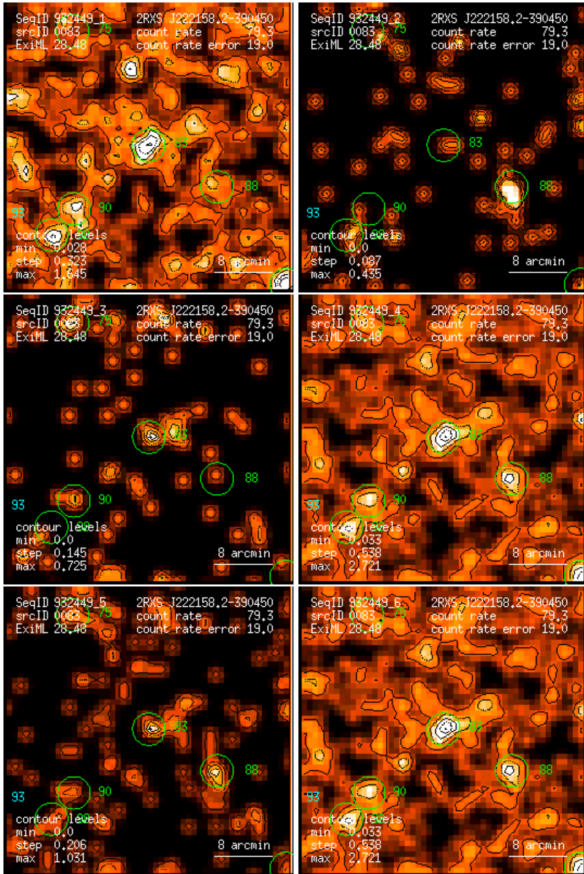
Figure 83: RASS 932449: detection 0083: band rate images, Gaussian filter: (1) PSPC channels 11 – 41, (2) 52 – 90, (3) 91 – 201, (4) 11 – 235, (5) 52 – 201, (6) 11 – 201. Broad band rates in counts/ks. Band rate contour levels in counts/ks/arcmin 2 .
