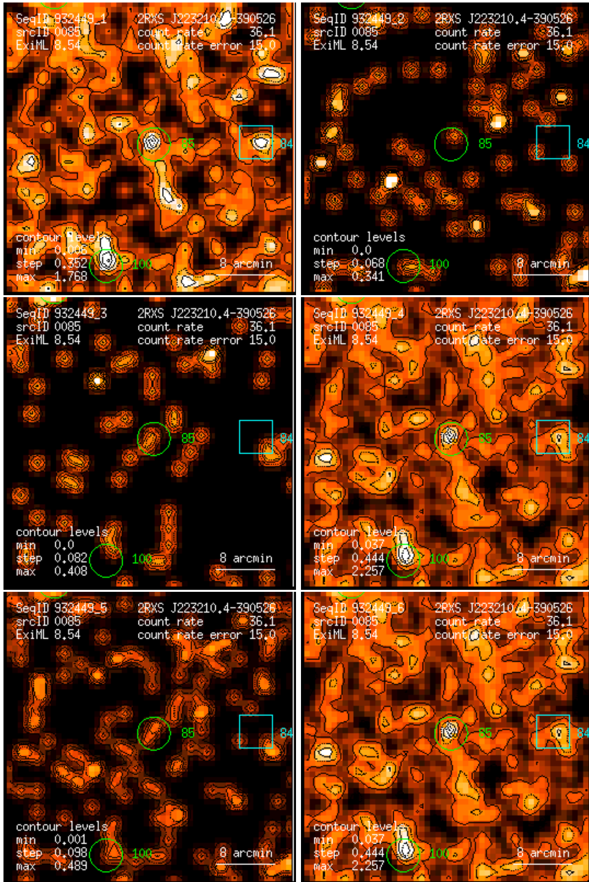
Figure 85: RASS 932449: detection 0085: band rate images, Gaussian filter: (1) PSPC channels 11 – 41, (2) 52 – 90, (3) 91 – 201, (4) 11 – 235, (5) 52 – 201, (6) 11 – 201. Broad band rates in counts/ks. Band rate contour levels in counts/ks/arcmin 2 .
