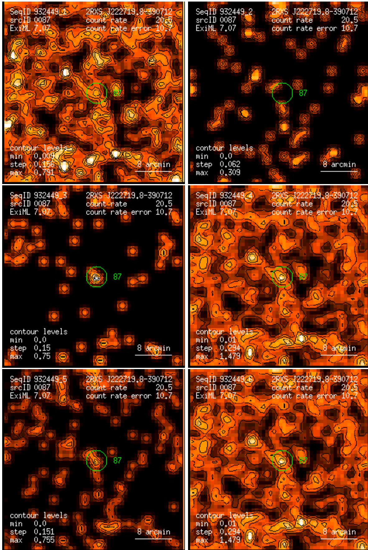
Figure 87: RASS 932449: detection 0087: band rate images, Gaussian filter: (1) PSPC channels 11 – 41, (2) 52 – 90, (3) 91 – 201, (4) 11 – 235, (5) 52 – 201, (6) 11 – 201. Broad band rates in counts/ks. Band rate contour levels in counts/ks/arcmin 2 .
