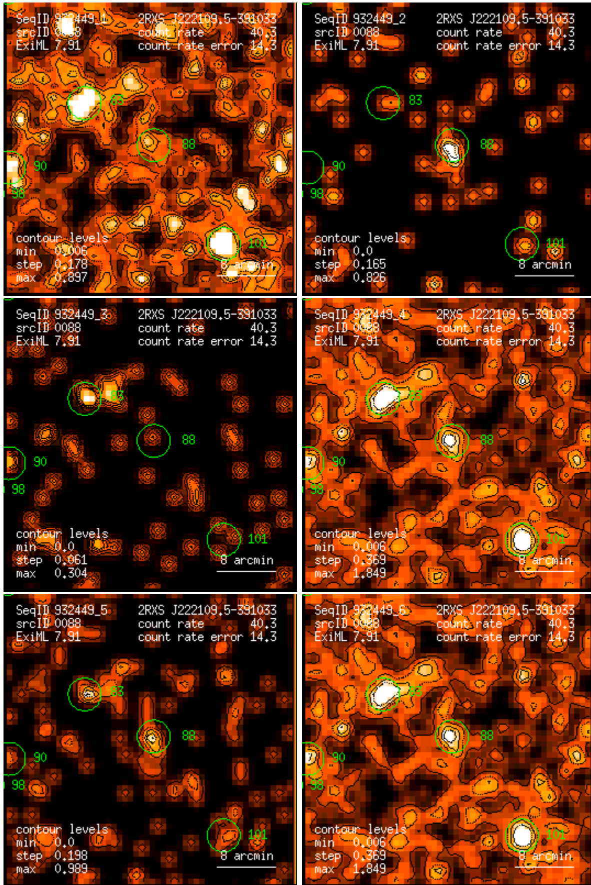
Figure 88: RASS 932449: detection 0088: band rate images, Gaussian filter: (1) PSPC channels 11 – 41, (2) 52 – 90, (3) 91 – 201, (4) 11 – 235, (5) 52 – 201, (6) 11 – 201. Broad band rates in counts/ks. Band rate contour levels in counts/ks/arcmin 2 .
