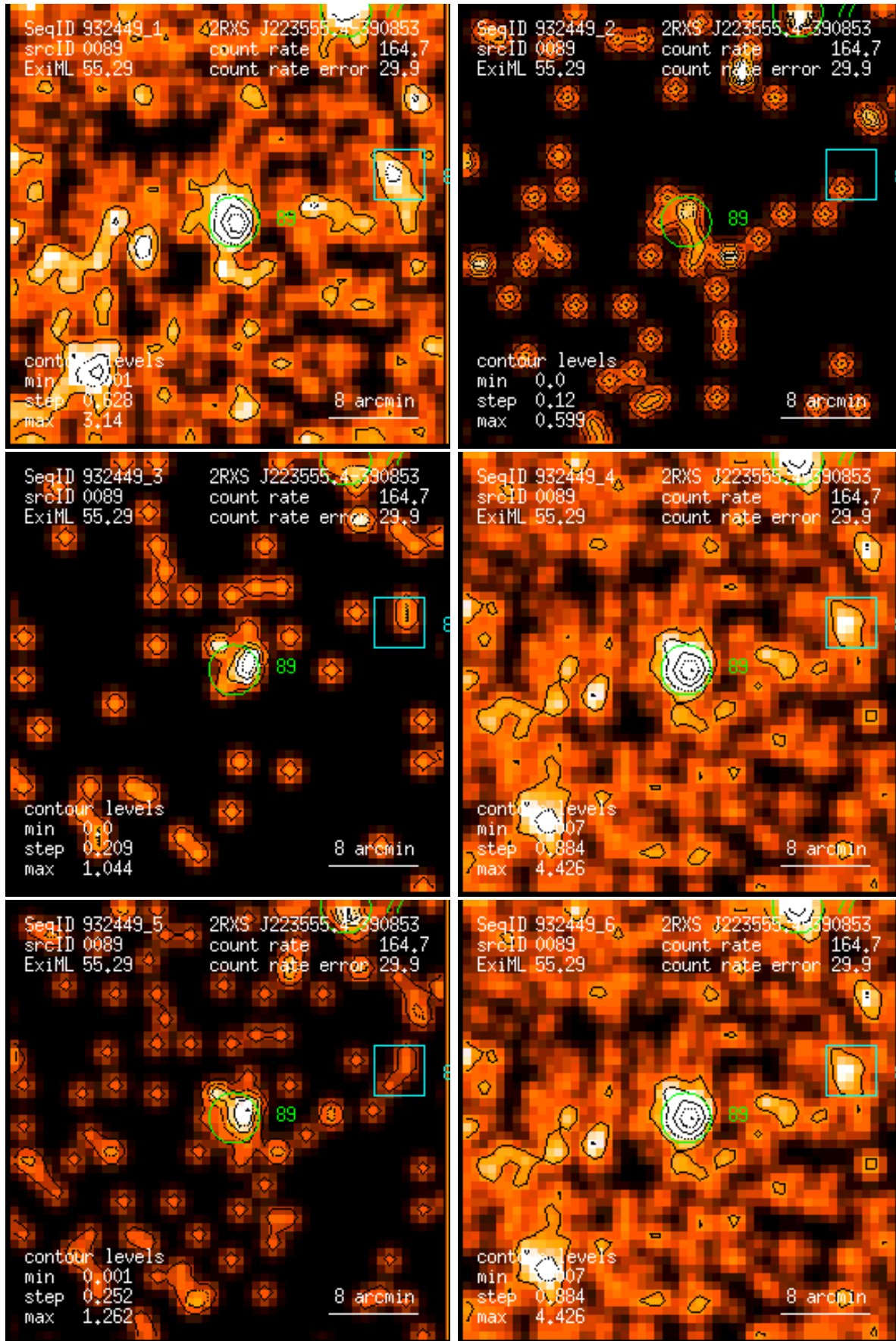
Figure 89: RASS 932449: detection 0089: band rate images, Gaussian filter: (1) PSPC channels 11 – 41, (2) 52 – 90, (3) 91 – 201, (4) 11 – 235, (5) 52 – 201, (6) 11 – 201. Broad band rates in counts/ks. Band rate contour levels in counts/ks/arcmin 2 .
