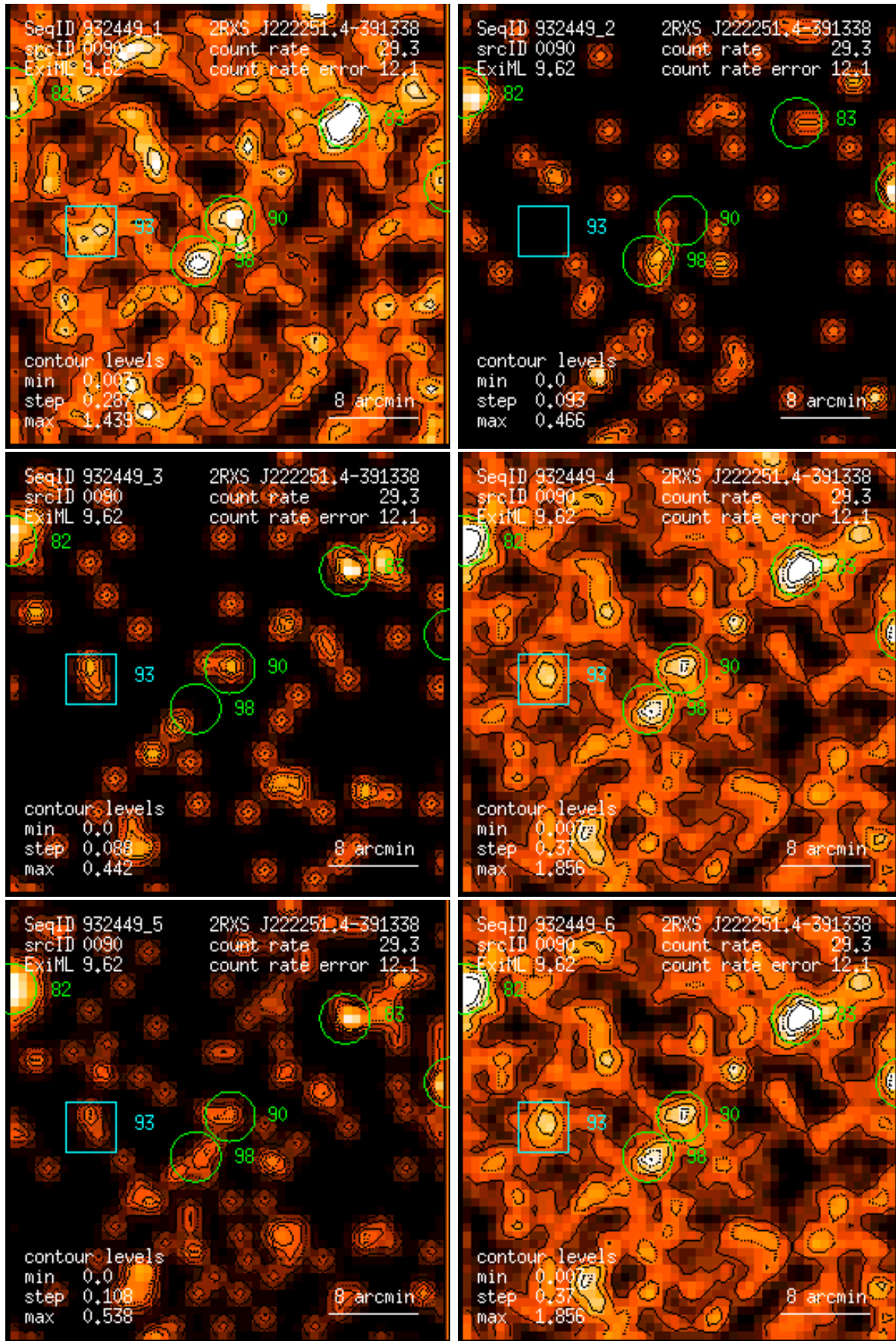
Figure 90: RASS 932449: detection 0090: band rate images, Gaussian filter: (1) PSPC channels 11 – 41, (2) 52 – 90, (3) 91 – 201, (4) 11 – 235, (5) 52 – 201, (6) 11 – 201. Broad band rates in counts/ks. Band rate contour levels in counts/ks/arcmin 2 .
